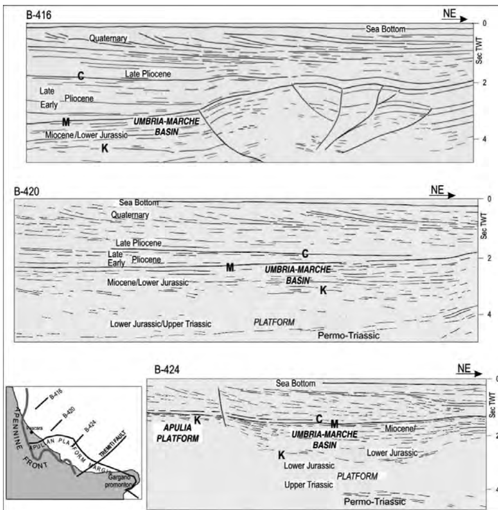
Fig. 3 - Line-drawing of three seismic profiles, normal to the Italian shore, in the central Adriatic Sea. Progradational sequence is highlighted by oblique shallow reflectors in the Quaternary sequence. C is a reflector in the Late Pliocene, M is the base of the Plio-Quaternary sequence, K is the top of the carbonate platform. Profiles, positioned in the map, depict different foreland behaviors in front of the Apennine Chain: profile B-416 shows a foreland, mainly covered by the pelagic sequence of the Umbria-Marche basin, westward tilted during the Lower Pliocene, folded and thrust by compression during the Late Pliocene. Profile B-420, near the northern margin of the Apulia carbonate platform, shows a minor tilting without folding. Profile B-424 shows the Apulia platform with its margin and the pelagic basin, without evidence of tilting: during the Upper Pliocene/Lower Pleistocene, the Apennine compressional structures are confined to in the inner onshore sector of the platform.
