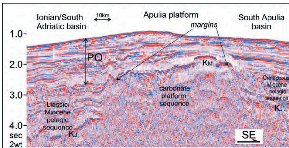
Fig. 5 – Part of the seismic profile MS-29 in the Otranto Channel (location in Fig. 1) across the Apulia carbonate platform (top marked with KM) and the contiguous pelagic domains of the Ionian/south Adriatic basin, to the north, and of the south Apulia basin, to the south. Platform and basins overlie the Upper Triassic/Jurassic platform (top marked with KJ). The Plio-Quaternary sediments (PQ) cover the pre-existing structures.
