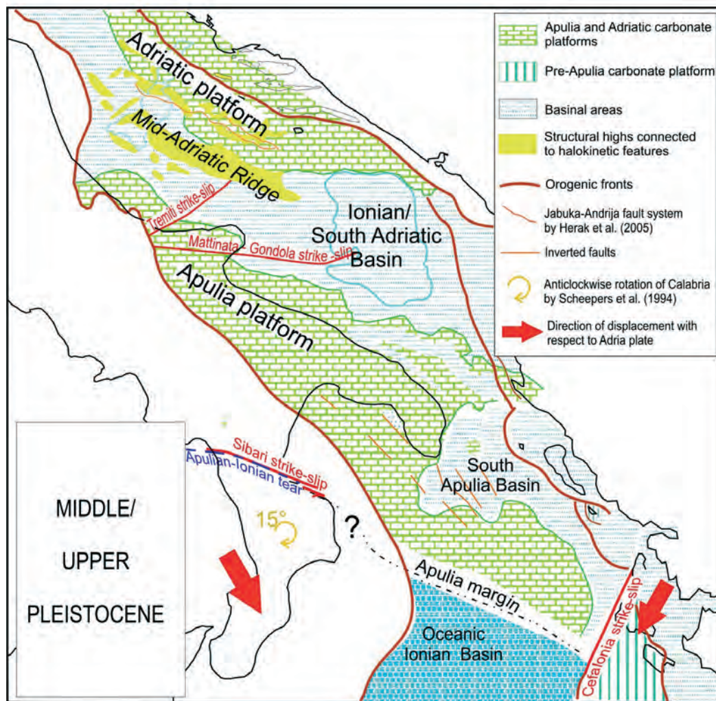
Fig. 10 - Map of the tectonic features active during the Middle/Upper Pleistocene in the study area: the margins of Dinaric (from Grandic et al. , 2001), NE-Apulia (from Argnani et al. , 1996; Nicolai and Gambini, 2007) and SE-Apulia (from Del Ben et al. , 2010) shallow platforms are outlined. Main halokinetic structures in the central Adriatic basin (from Geletti et al. , 2008) depict the Mid-Adriatic Ridge. The orogenic fronts of Dinarides (from Grandic et al. , 2001), Albanides (from Del Ben et al. , 1994; Argnani et al. , 1996), Hellenides (from Kokinou et al. , 2005) and southern Apennines (CNR-Progetto Finalizzato Geodinamica, 1991) are indicated. The two arrows highlight the direction of migration of the Calabrian Arc (from Del Ben et al. , 2008) and of the SW-Hellenic Arc (from Khale et al. , 1995).
