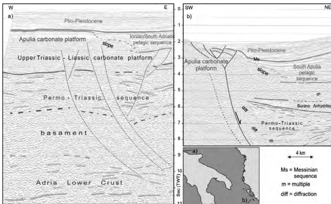
Fig. 2 – Deep-reflection profiles across the Apulia platform margin. a) western part of the CROP-M13 profile, on the northern offshore of the Gargano promontory. The carbonate platform lies above the well-reflecting Permo-Triassic sequence. The Liassic-Tertiary platform/basin transition seems controlled by a reactivation of the Permo-Triassic normal fault system. This last terminates on the top of the deformed and thinned lower crust, fracturing, thinning and tilting the basement. b) ENE part of the CROP-M34 profile, in the offshore of the Ionian Island. The Permo-Triassic sedimentary wedge suggests a coeval tectonic activity of normal faults, successively reactivated, to separate the carbonate and the pelagic domains.
