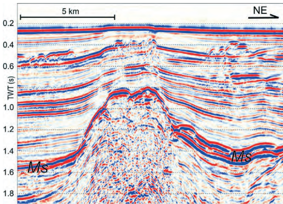
Fig. 4 – Detail of the seismic profile CROP-M15 crossing the Mid-Adriatic Ridge (position in Fig. 1): the gentle bathymetric high of the ridge is connected to a deep structure, due to a halokinetic feature.
