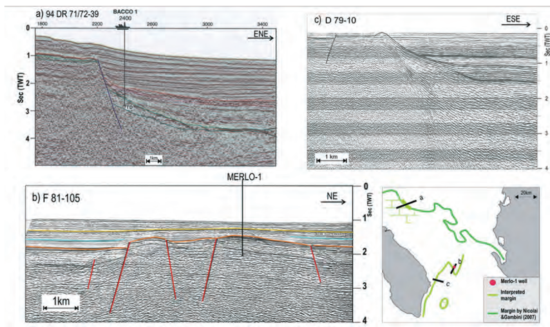
Fig. 6 – Seismic profiles crossing the Apulia platform margin in the east Salento offshore (location in Fig. 1 and in the inset). In a) the margin between the platform and the Ionian/south Adriatic basin is evident. In b) the platform is calibrated by the Merlo-1 borehole. In c) the margin between the platform and the south Apulia basin is also clearly depicted by reef and slope features.
