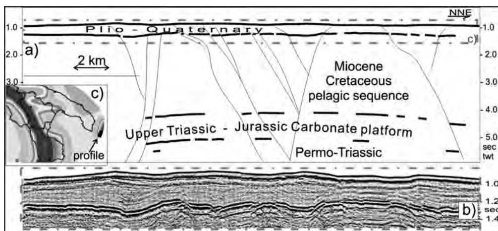
Fig. 7 – Part of the seismic profile F-55 (position in Fig. 1): inversion tectonics in the south Salento offshore [modified by Del Ben (2010)]. a) schematic line-drawing of the profile: here the interpretation shows a system of normal faults cutting the base of the Plio-Quaternary sequence. b) the upper part of the profile, with a vertical exaggeration x6, highlights typical morphologies of the area with gentle swells of shallow sediments and of the sea-floor: they are focused on the graben or structural minima defined by the normal faults. This morphology was interpreted as a consequence of inversion tectonics that rotate previous normal faults, uplift rigid blocks and fold and uplift shallow sediments. c) a relatively high seismic risk area [maximum value of acceleration at bedrock by INGV (2006)] was recognized in the area involved in this deformational style.
