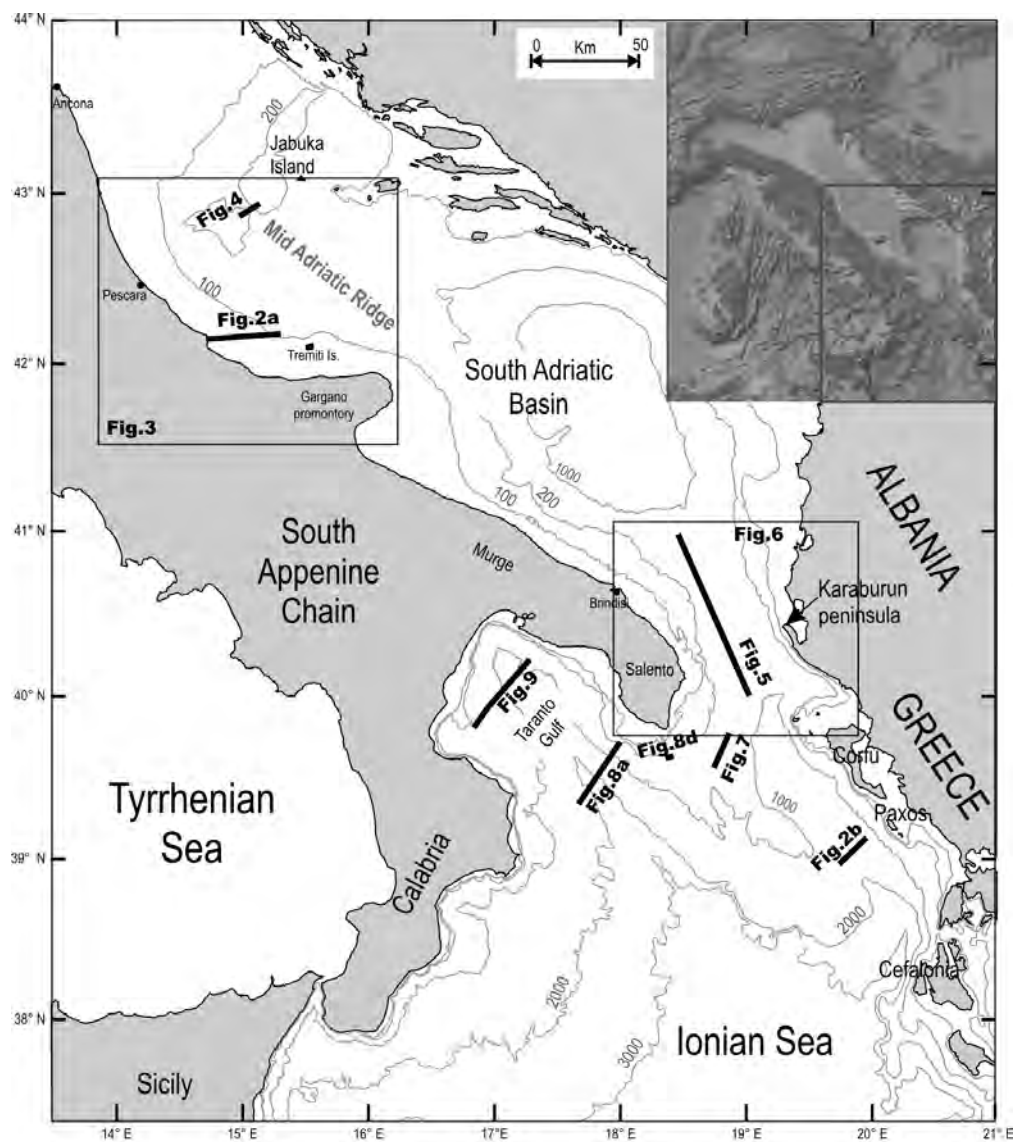
Fig. 1 - Map of the investigated area. Seismic profiles present in the relevant figures are indicated.
