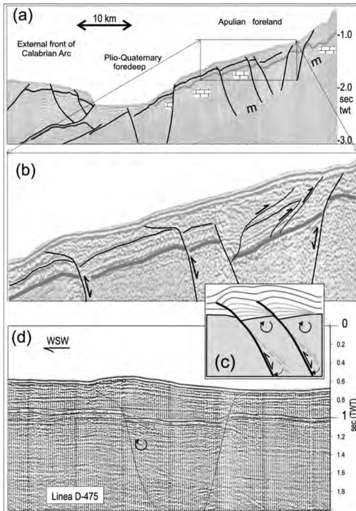
Fig. 8 – a) part of the seismic profile MS-26: a normal fault system related to the Pliocene-Lower Pleistocene bending phase. b) the detail shows how recent, normal faults have been inverted, producing the gentle swelling of shallow soft sediments; c) outline of the effects of inversion tectonics in the area: the new compressive regime produces the rotation of previous normal faults, back-rotation and uplift of rigid fault blocks, uplift, folding and thrusting of shallow soft sediments (after Wang et al. , 1995); d) detail of seismic profile D-475: inversion tectonics generally seem to involve particularly E-dipping normal faults, which are more oblique, producing a back-thrust (NW-vergence), with respect to the direction of migration of the Calabrian Arc. Location of sections in Fig. 1.
