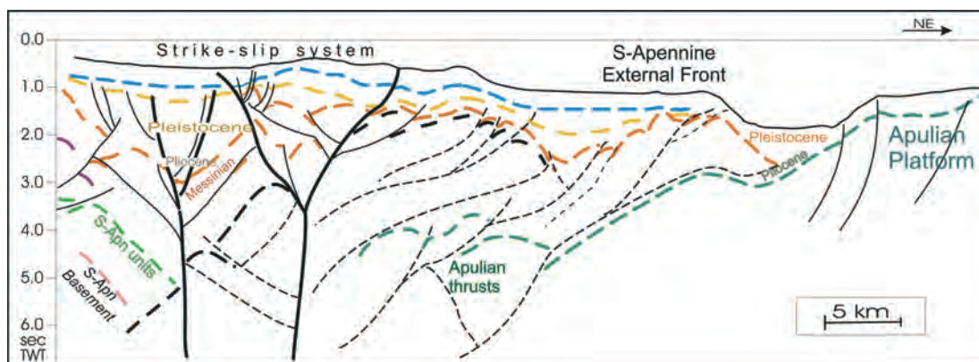
Fig. 9 - Line-drawing of a NE-SW profile in the Taranto Gulf [modified after Del Ben et al. (2008)]. The deep Plio-Pleistocene basin on the left was originated by transtensional tectonics of the Sibari strike-slip fault, the Apulian/Ionian tear fault, that separated the buoyant continental crust from the oceanic crust subsiding below the Calabrian Arc is supposed to be located below it. The crust underneath the Apulia platform, detached from the Ionian crust, thrusts below the South Apennine units.
