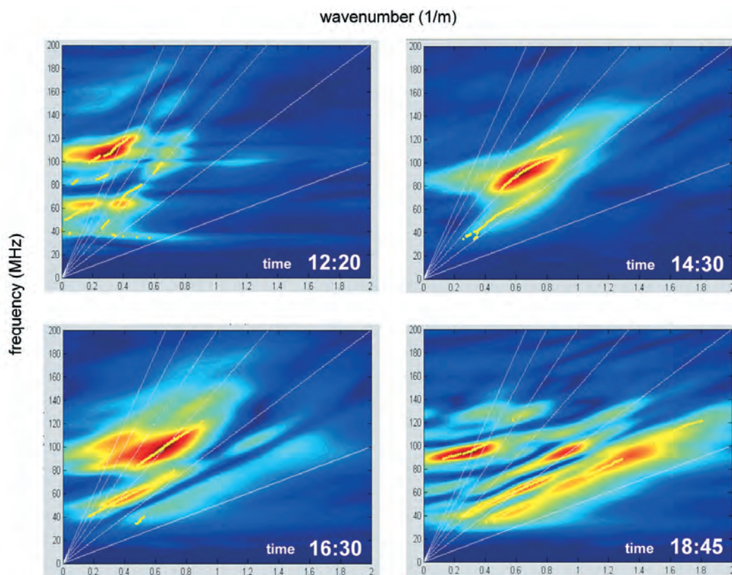
Fig. 7 - f - k spectra corresponding to the four radargrams in Fig. 5. The absolute maxima at each frequency are marked with a yellow dot. The white lines indicate different apparent velocity values and are displayed for reference.
