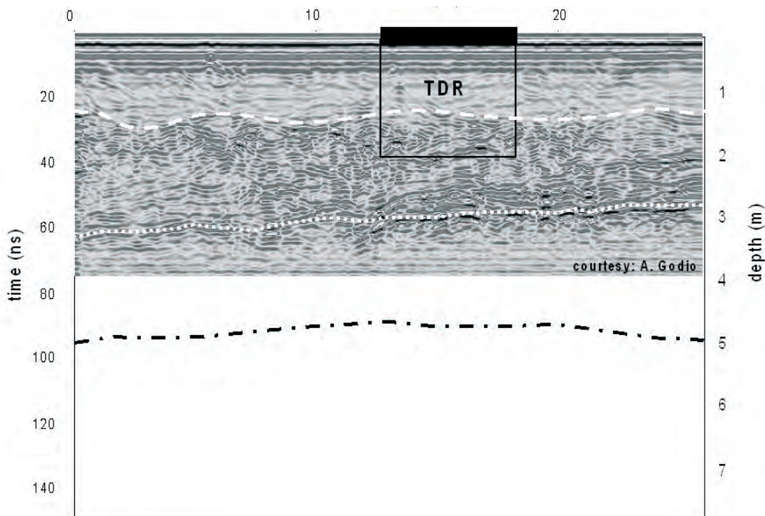
Fig. 4 - Minimum offset GPR reflection survey (450 MHz) collected under natural conditions at the Grugliasco site (courtesy Alberto Godio, Polytechnic of Turin).
