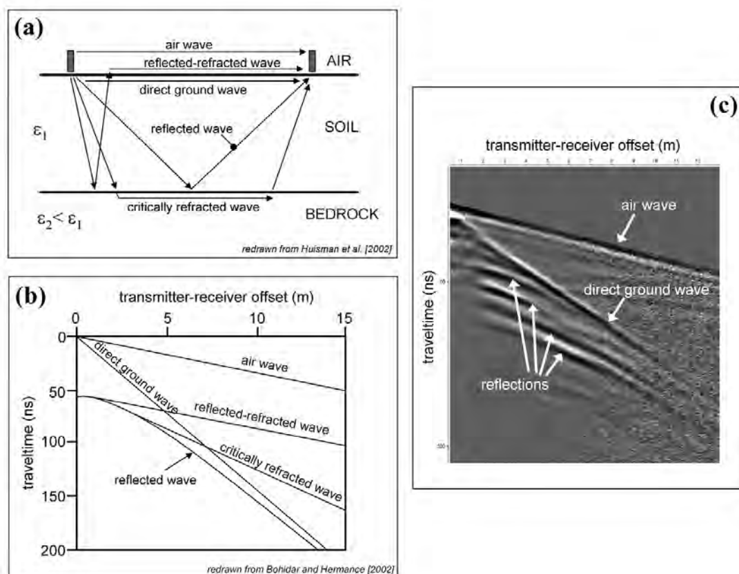
Fig. 1 - (a) expected GPR wave propagation pathways in surface-to-surface configuration; (b) corresponding time-offset relationships; (c) example field data under natural conditions from the Grugliasco site (March 2004).
