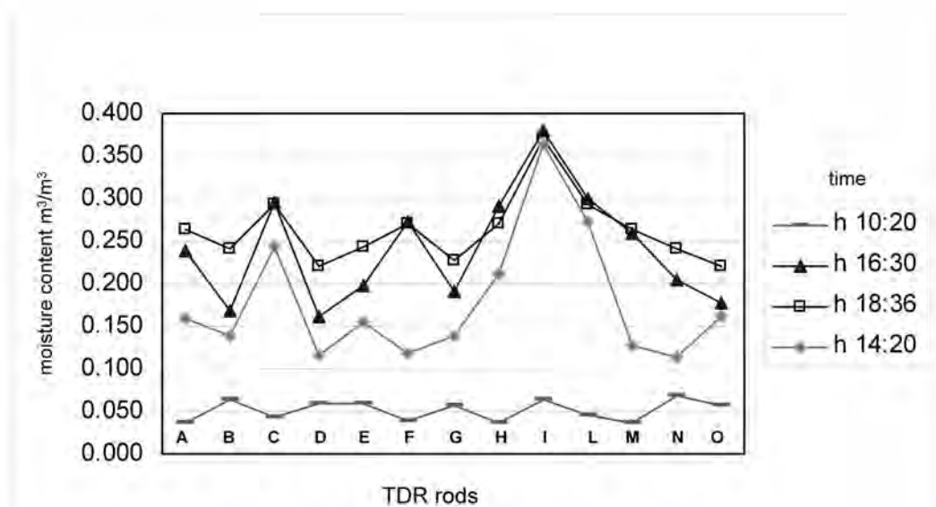
Fig. 10 - Soil water content values from TDR measurements at the four instants in time during irrigation at the Grugliasco site; for the location of each probe, see Fig. 2.
