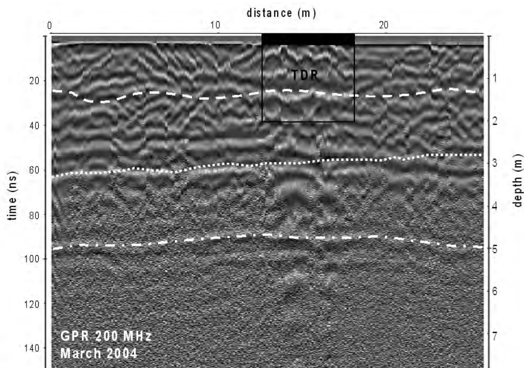
Fig. - 3: Minimum offset GPR reflection survey (200 MHz) collected under natural conditions at the Grugliasco site. Note the location of the TDR probes relative to the overall survey line.
