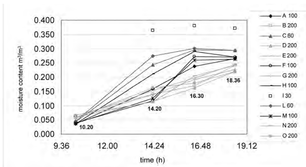
Fig. 11 - Soil water content values from TDR measurements at the four instants in time during irrigation at the Grugliasco site; for the location of each probe, see Fig. 2.
