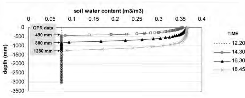
Fig. 12 - Soil water content profiles simulated using a 1D infiltration model calibrated on the location of the infiltration front as indicated by GPR measurements (see Table 1) using the unsaturated flow parameters in Table 2.
