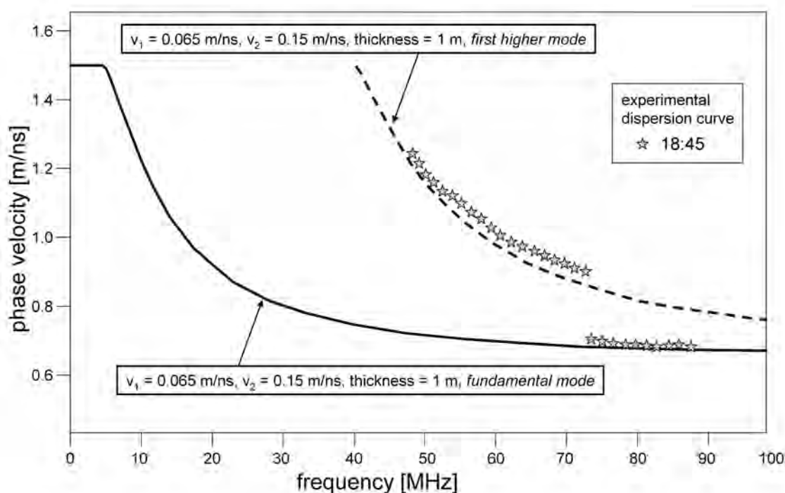
Fig. 8 - Experimental dispersion curves corresponding to the radargram at 18:45 in Fig.5, compared with an expected simulated dispersion curve produced with parameters similar to the observed velocities and thickness during the Grugliasco irrigation experiment. Note the strong discrepancy (except at high frequencies) between experimental and modelled data for the fundamental mode, while the simulation of the first higher mode may match the lower frequency part of the curve.
