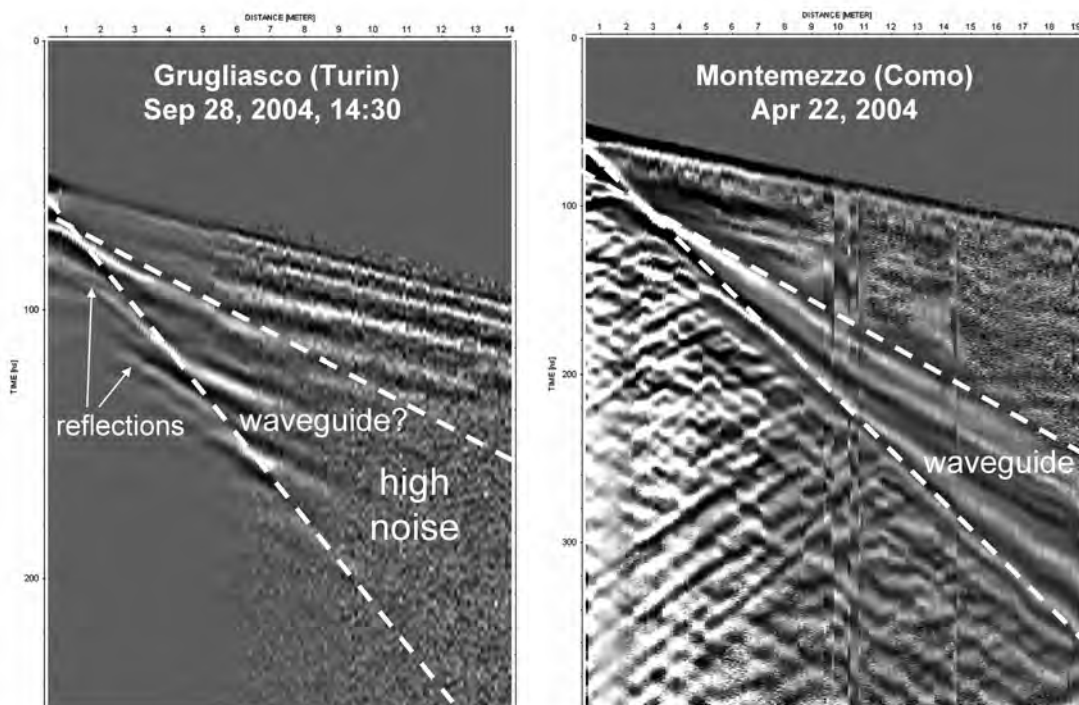
Fig. 6 - Comparison between GPR WARR data collected at Grugliasco 2 hours after the start of irrigation (left panel) and the data collected at the Montemezzo site (Como) in April 2004. In the Montemezzo data, the events to the right of the waveguide energy are interpreted as energy travelling horizontally and reflected back by discontinuities in the bedrock.
