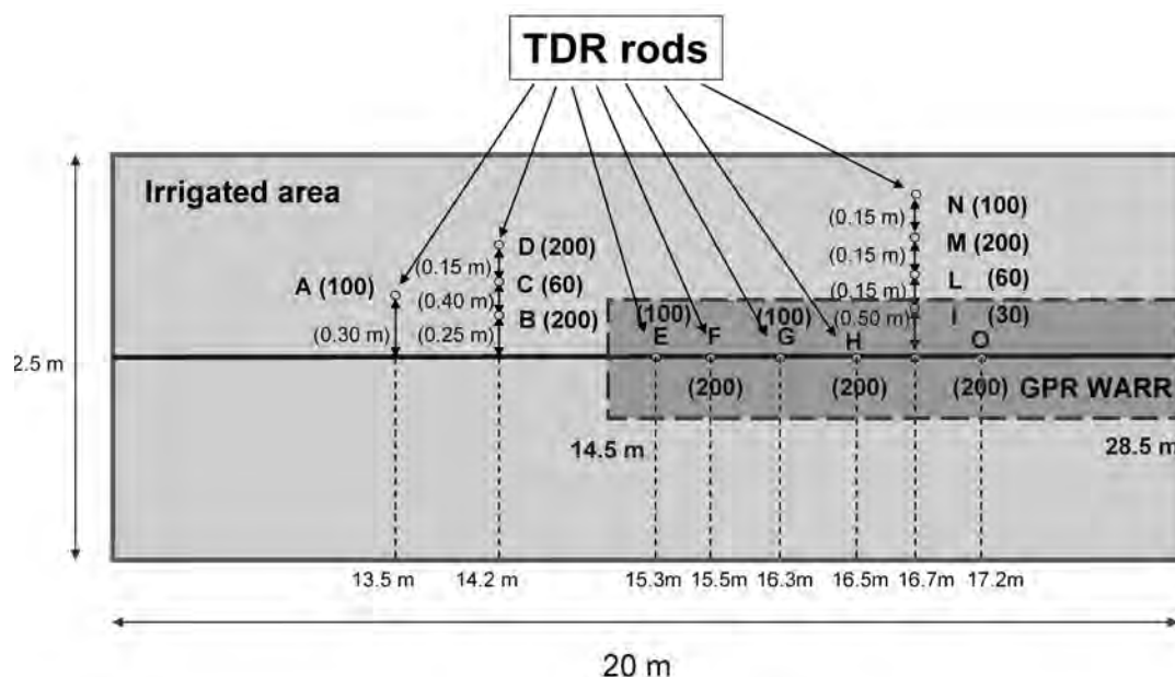
Fig. 2 - Grugliasco site: sketch of the measurement area with TDR locations (the numbers indicate the rod lengths in cm), GPR survey area (dark grey) and irrigated area (light grey).
