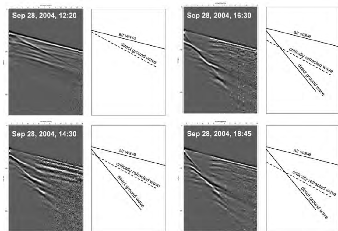
Fig. 9 - Interpretation of the four radargrams acquired during irrigation using a simplified approach that assimilates the data to critically refracted events.
