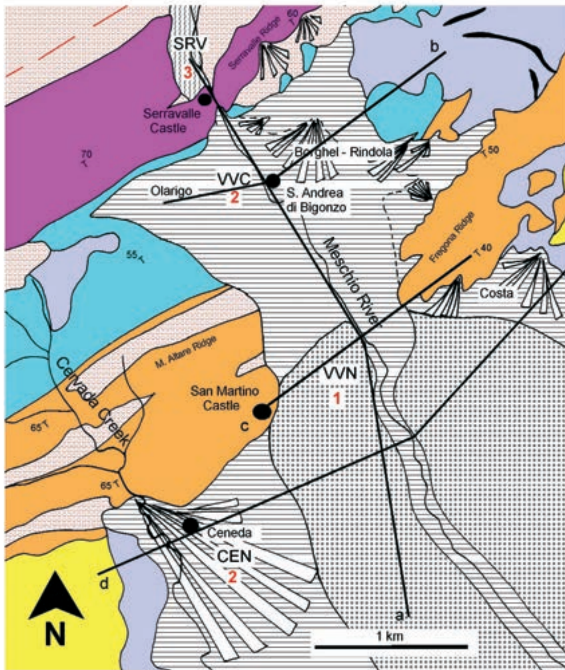
Fig. 1 - Detailed geo-lithological map of the Vittorio Veneto area. Pre-Quaternary succession (Southalpine Molasse, Upper Oligocene - Pliocene pp): violet: calcarenites; light blue: marls; orange: arenites and conglomerates; yellow: pelites and sandstones. Quaternary deposits: violet: glacial deposits; vertical line: sands with local lacustrine silts and peat levels; ruled: fine alluvial and colluvial deposits; circles: coarse alluvial deposits; red dotted: detrital talus; red sketched line: fault. Black heavy line: geological cross sections. SRV: Serravalle; VVC: Vittorio Veneto centre; VVN: Vittorio Veneto modern city and CEN: Ceneda. Relative red numbers refer to identified geological soils (see text for explanation).
