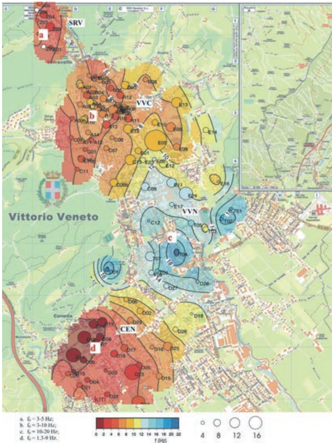
Fig. 3 - HVSR amplitude of the peak in the frequency range 0.5-22 Hz. The colour and size of the circles indicate peak frequency and amplitude of the HVSR, respectively. White circles indicate sites with very low H/V amplitude or flat response. The value of the resonance frequency is also indicated along the iso-frequency lines computed by interpolating the peak frequencies. Letters and numbers refer to the zonation based on HVSR resonant frequencies and types of soils (see text), respectively.
