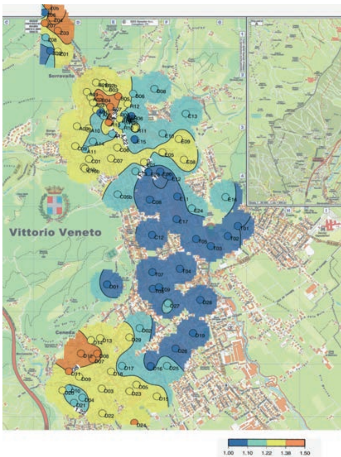
Fig. 4 - Microtremor HVSR mean amplitude over the frequency band [0.8, 8] Hz.
