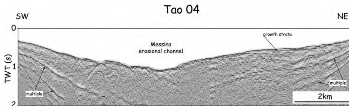
Fig. 4 - Seismic profile TAO 04 (stack) crossing the Messina Straits. Major sea-floor erosion and ensuing hard bottom contribute to deteriorating the quality of the seismic signal. Evidence of growth strata on a west-dipping fault, possibly not currently active, can be seen on the Calabrian side (NE). Profile acquired with the short streamer. Location in Fig. 2.
