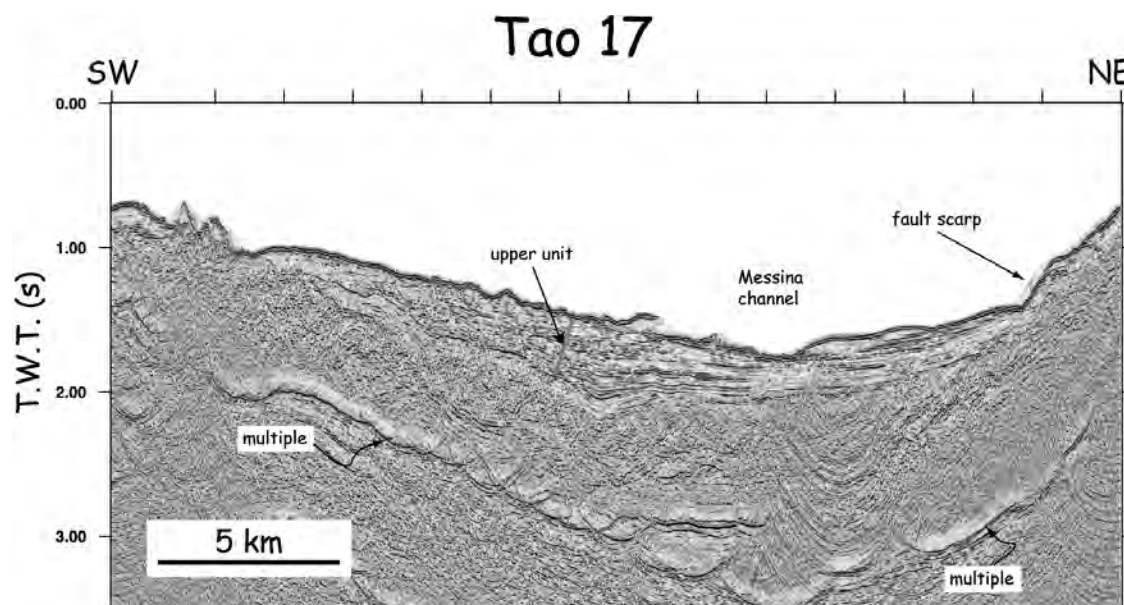
Fig. 6 - Seismic profile TAO 17 (migrated) showing the fault scarp on the Calabrian side (NE), whereas no major faulting affects the Quaternary sedimentary package over the rest of the profile. Profile acquired with the long streamer. See Fig. 2 for location.
