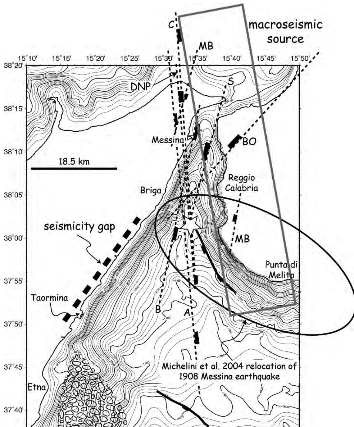
Fig. 2 - Map showing the location of the fault identified offshore southern Calabria through the Taormina-2007 seismic survey. The star indicates the epicentre of the Messina 1908 earthquake according to Schick (1977), whereas the dashed lines show suggested fault planes for the same event, from various authors [S: Schick (1977), MB: Mulargia and Boschi (1983), BO: Bottari et al. (1986), C: Capuano et al. (1988), B: Boschi et al. (1989), DNP: De Natale and Pingue (1991), A: Amoruso et al. (2002)]. The relocation of Michelini et al. (2004) and the macroseismic location (Gasperini et al. , 1999; DISS Working Group, 2006) for the Messina 1908 earthquake are also indicated. The seismicity gap is located after Neri et al. (2006). The gravel pattern next to Mt. Etna, indicating a chaotic seismic facies, and the adjacent fault are from Argnani and Bonazzi (2005).
