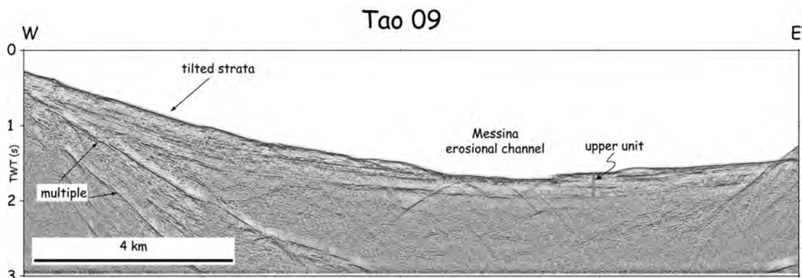
Fig. 3 - Seismic profile TAO 09 (stack) across the central part of the supposed Taormina fault. Note the 0.4–0.5 s (TWT) thick package of almost parallel strata dipping to the east on the slope and flattening further to the east (upper unit). Some minor onlaps occur at the very base of the package on the western slope. Profile acquired with the short streamer. See Fig. 2 for location.
