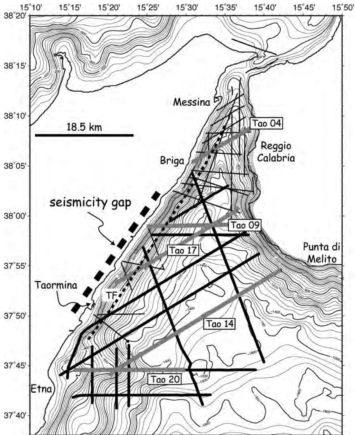
Fig. 1 - Map showing traces of seismic profiles in the study area. Bold black lines indicate the profiles acquired with the long streamer (see text for explanation), whereas profiles acquired with the short streamer are shown as thin black lines. The location of the seismicity gap (Neri et al., 2006) and of the inferred Taormina Fault (TF; Catalano and De Gudi, 2003) are also shown. The portions of seismic profiles shown in Figs. 2 to 6 are labelled and indicated with a thick gray line.
