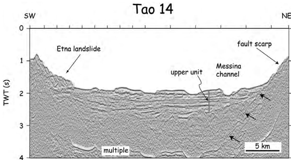
Fig. 5 - Seismic profile TAO 14 (migrated). Note the absence of faulting and the undisrupted Quaternary strata across most of the profile, whereas a fault scarp occurs on the Calabrian side (NE), with arrows indicating the fault plane. On the SW side the profile reaches the Etna submarine slide (see text). Profile acquired with the long streamer. See Fig. 2 for location.
