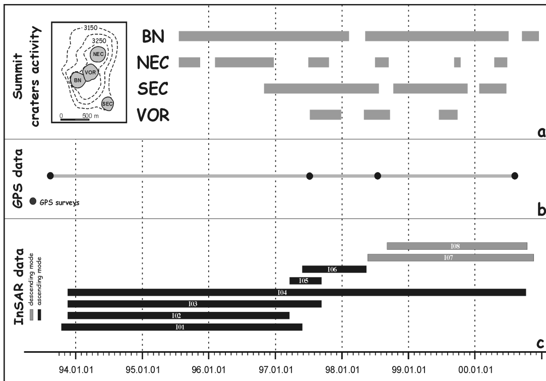
Fig. 2 - a) Graphic illustration of the activity at the summit craters during 1993-2000 (BN, Bocca Nuova; NEC, NE Crater; SEC, SE Crater; VOR, Voragine); b) time coverage for the GPS data; c) time coverage for InSAR data.
