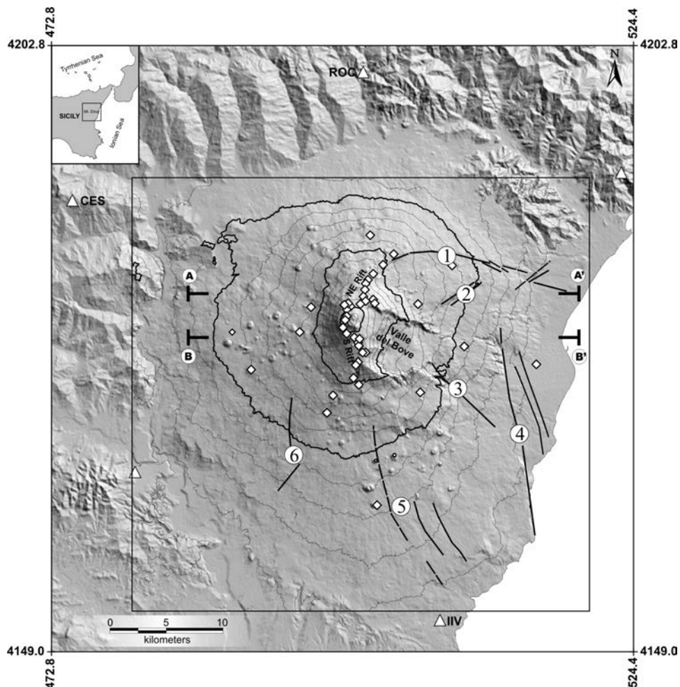
Fig. 1 - Structural sketch of Mt. Etna: 1) Pernicana fault; 2) Ripe della Naca fault; 3) Santa Venerina fault; 4) Timpe fault system and Moscarello fault; 5) Mascalucia-Tremestieri-Trecastagni faults system, 6) Ragalna fault. Mt. Etna GPS Network is also reported: diamond for inner benchmarks, triangle for external reference benchmarks. Coordinates in UTM projection, zone 33N. The box indicates the area shown in Figs 3, 4, 5, 6 and 7. A-A' and B-B' are schematic cross-sections reported in Fig 7.
