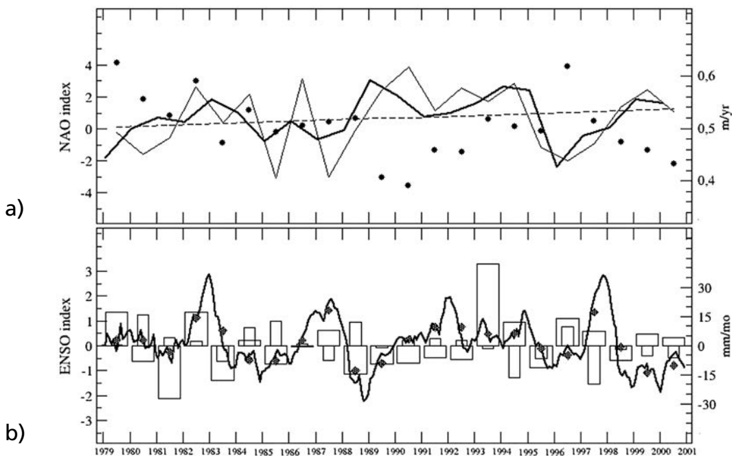
Fig. 3 - a) NAO indexes: annual (light line) and winter (solid line; the dashed line is the linear regression) between 1979 and 2000; DAAC-GPCP rainfall on Mediterranean Sea (dots). b) ENSO indexes: Niño3.4 monthly (solid line); Niño3.4 annual (diamonds) between 1979 and 2000; DAAC-GPCP precipitation anomalies with respect to the climatological mean on western Mediterranean Sea during September-October-November (SON, large bars) and March-April-May (MAM, narrow bars).
