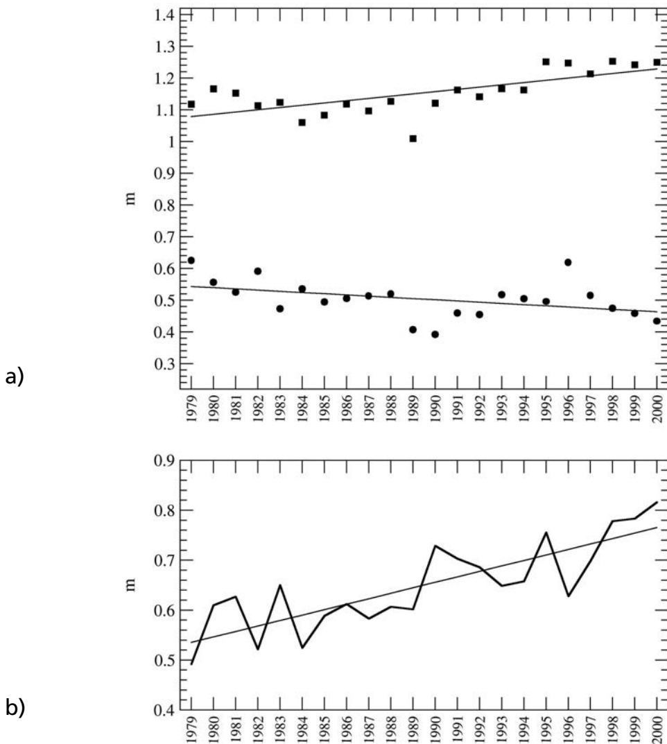
Fig. 2 - a) DAAC-GPCP precipitation (●), NCEP/NCAR evaporation (■), with respective linear regressions. b) E-P evolution on Mediterranean Sea between 1979 and 2000 with linear regression.
