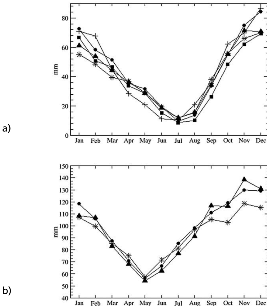
Fig. 1 - Monthly averages of precipitation on Mediterranean Sea: a) DAAC-GPCP mean between 1979 and 2000 (▲), DAAC-GPCP mean between 1988 and 1996 (*), HOAPS mean between 1988 and 1996 (+), Legates climatology between 1920 and 1980 (■), Jaeger climatology between 1955 and 1965 (●); b) NCEP climatology between 1948 and 2000 (●), NCEP mean between 1988 and 1996 (▲), HOAPS mean between 1988 and 1996 (*).
