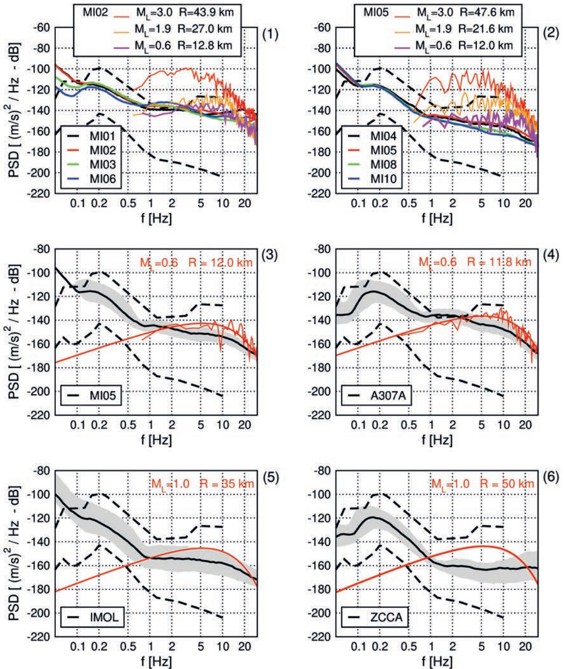
Fig. 10 - Validation of results: examples of simulated and recorded power spectra. Panel 1: mean horizontal component of velocity power spectra recorded at surface station MI02. Panel 2: mean horizontal component of velocity power spectra recorded at borehole station MI05. Power spectra of the recorded events, having magnitudes 0.6, 1.9, and 3.0, are compared with the median PDF of the ambient seismic noise, recorded with surface and borehole stations (panels 1 and 2, respectively). Panels 3 and 4: mean horizontal component of recorded and simulated power spectra for the M_L 0.6 event localised in the IDD. For the borehole station MI05 (panel 3) and the surface station A307A (panel 4) the earthquake power spectra are compared with the corresponding PDF of the observed ambient seismic noise. Panels 5 and 6: power spectra of a M_L 1.0 event hypothetically located at the centre of the reservoir, and simulated at stations IMOL (Po Plain - borehole) and ZCCA (Apennines - surface). Simulated PSD are compared with the corresponding PDF of observed ambient seismic noise. Dashed lines: NHNM and NLNM curves of Peterson (1993).
