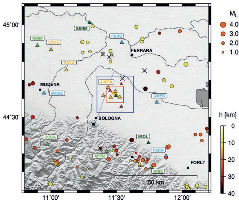
Fig. 9 - Seismicity recorded by the MISN in the period 1 January 2018 - 31 March 2019. Earthquake with epicentral distance less than 50 km are shown. Circle dimensions are proportional to the magnitude, colours indicate the event depth. Seismic events not included in the catalogue of the ISN are marked with crosses. Other symbols are as in Fig. 1.
