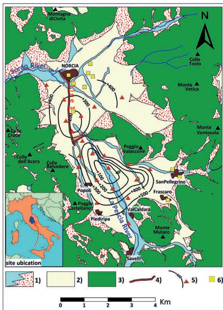
Fig. 1 - Geological map of the NIB (modified from: Motti et al. , 2014) and previous geophysical surveys: 1) fluvio-lacustrine, slope deposits (Holocene); 2) fluvio-lacustrine deposits (Pleistocene-Holocene); 3) calcareous-siliceous-marly deposits (Meso-Cenozoic); 4) seismic lines by Böhm et al. (2011); 5) VES and bedrock elevation in metres a.s.l., by Biella et al. (1981); 6) HVSR and arrays by Regione Umbria (2018).
