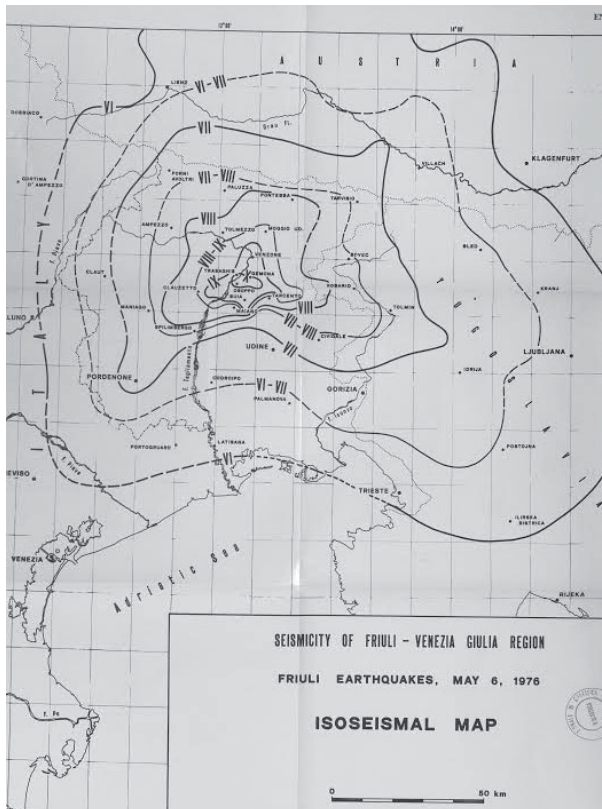
Fig. 2 - Isoseismal map for Italy: a) compiled by Gasparini (1976); b) compiled by Giorgetti (1976).
