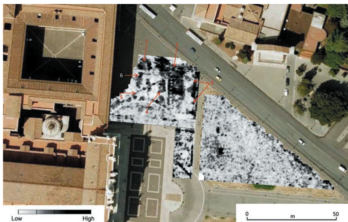
Fig. 7 - St. John Lateran square. Area A2, B2 and C2, GPR 400 MHz, slices at the estimated depth of 1.35 m.
