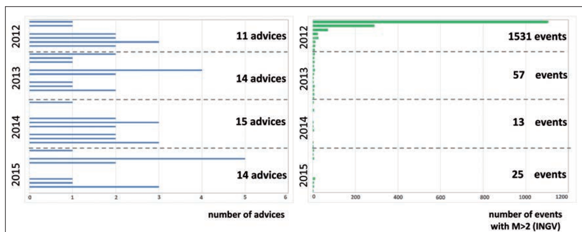
Fig. 12 - Temporal relationships between reports of anomalous geological phenomena and seismicity (inside.rm.ingv.it) in the area struck by the 2012 seismic swarm.
