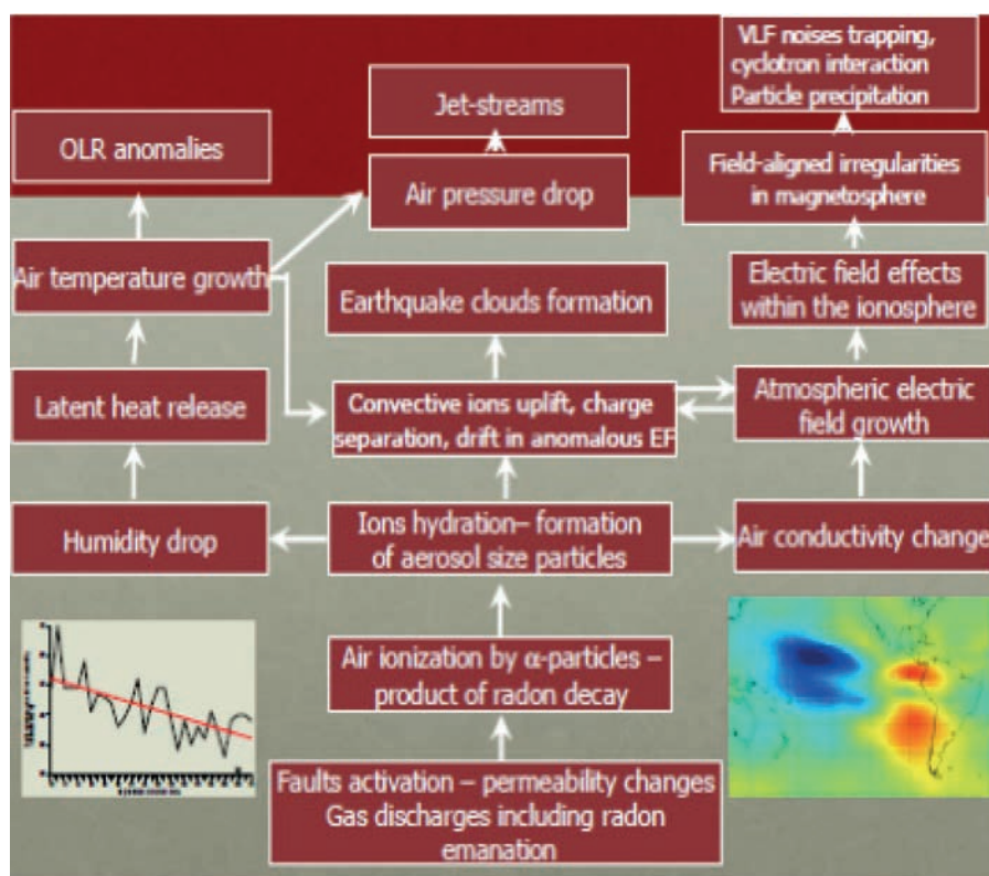
Fig. 11 - The physical model proposed by Pulinet (2009) named LAIC [Lithosphere-Atmosphere-Ionosphere Coupling; adapted from Pulinet (2009)].
