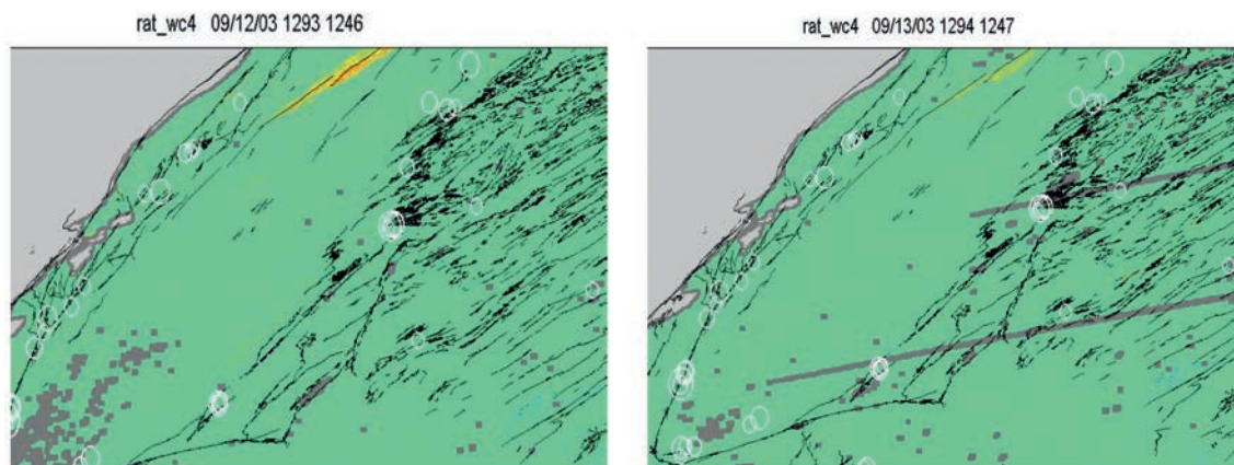
Fig. 7 - Anomalously high RETIRA values (in yellow) associated with Corning and Great Valley fault zones on the northern edge of the tile (from Eneva et al. , 2008), on two consecutive days (straight grey lines are data errors).
