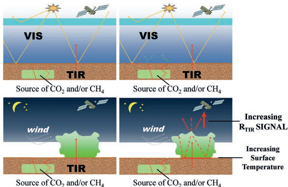
Fig. 8 - Physical model proposed by Tramutoli et al. (2001, 2005, 2013). In the preparatory phases of an earthquake, greenhouse gases, like \text{CO}_2 and \text{CH}_4 , can reach the lower part of the atmosphere as consequence of their migrations through the fractures. These can locally operate like greenhouse gases, producing in this way an increase of TIR signal which is emitted by the Earth and measured by satellite sensors (adapted from Tramutoli et al. , 2013).
