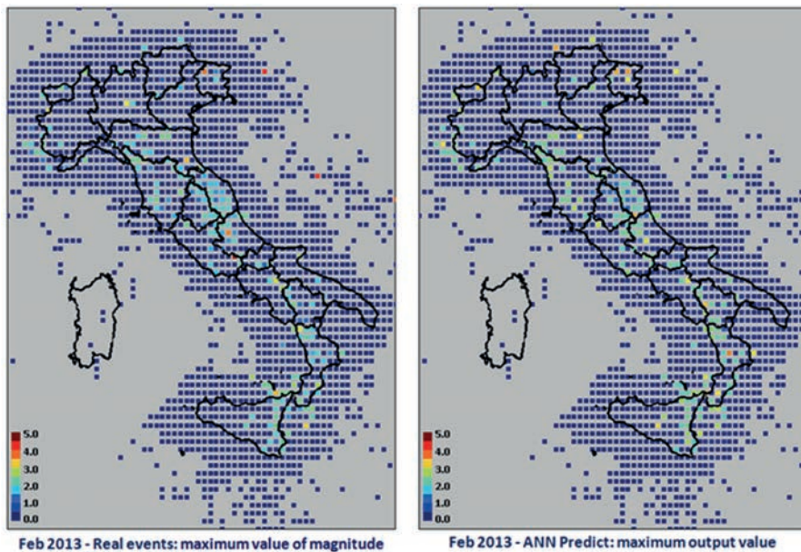
Fig. A8 - Results of February 2013: a) maximum magnitude of real events; b) maximum magnitude predicted by ANN.
