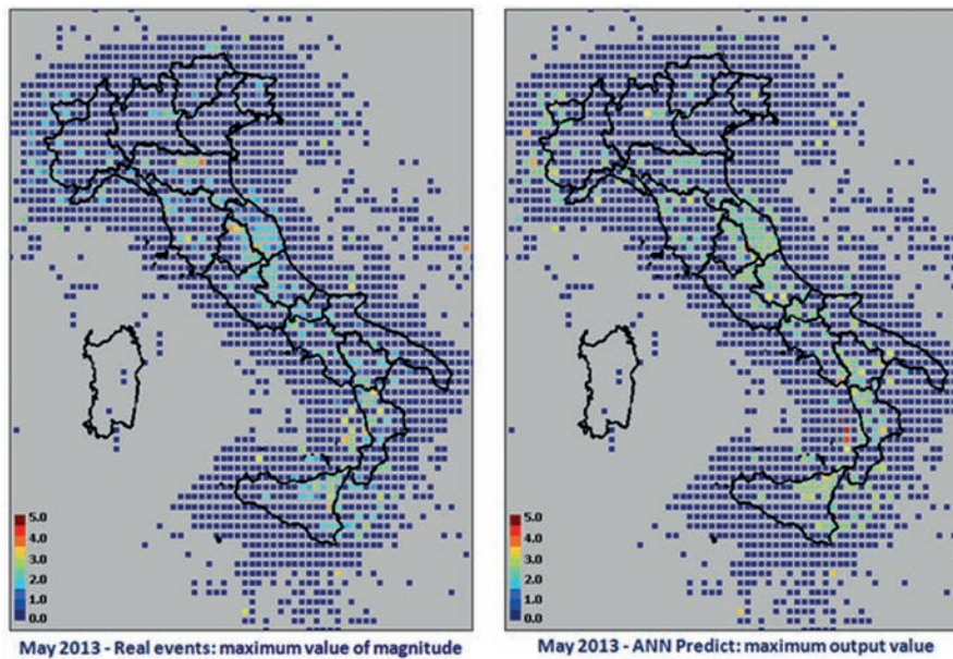
Fig. A11 - Results of May 2013: a) maximum magnitude of real events; b) maximum magnitude predicted by ANN.
