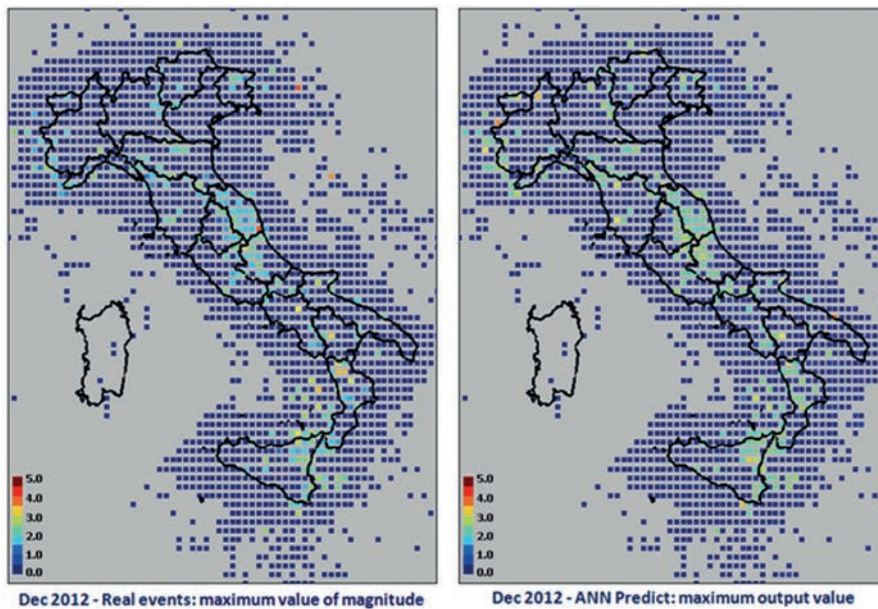
Fig. A6 - Results of December 2012: a) maximum magnitude of real events; b) maximum magnitude predicted by ANN.
