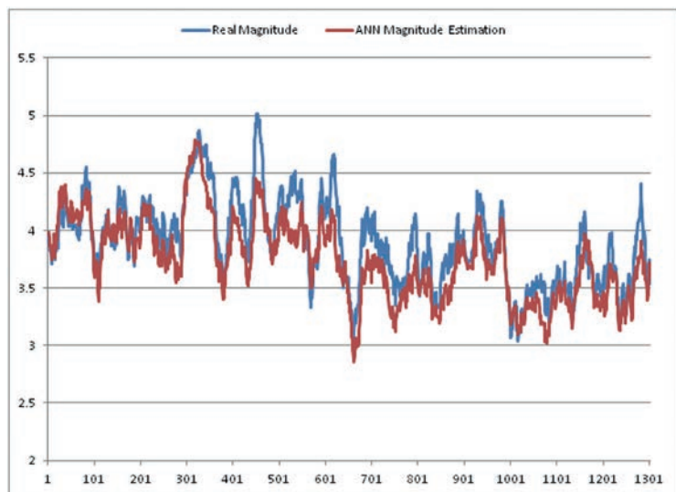
Fig. 4 - Mobile average of the real magnitude and of the ANN estimation of the events in 2011 recorded by USGS and ISIDE catalogues.
