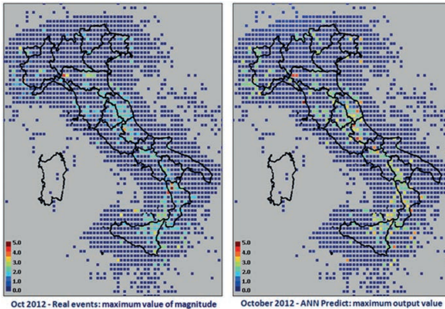
Fig. A4 - Results of October 2012: a) maximum magnitude of real events; b) maximum magnitude predicted by ANN.
