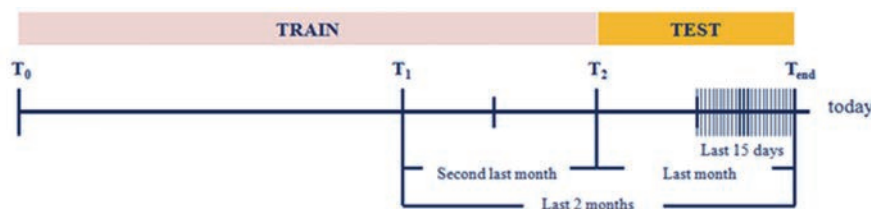
Fig. 5 - Explanation of the pre-processing coding system adopted to increase the 7 input variables of the data set into 15, in order to make daily prediction for each of the 2054 boxes of the assumed grid.
