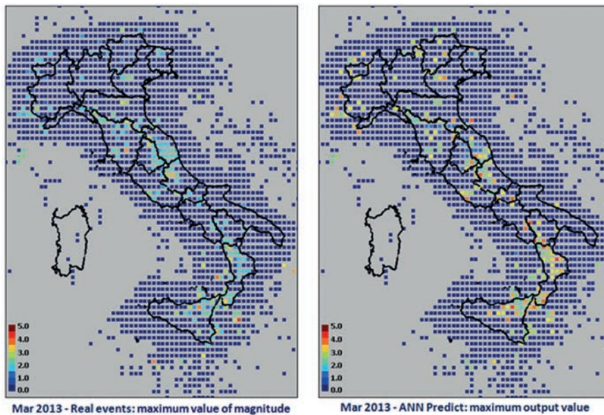
Fig. A9 - Results of March 2013: a) maximum magnitude of real events; b) maximum magnitude predicted by ANN.
