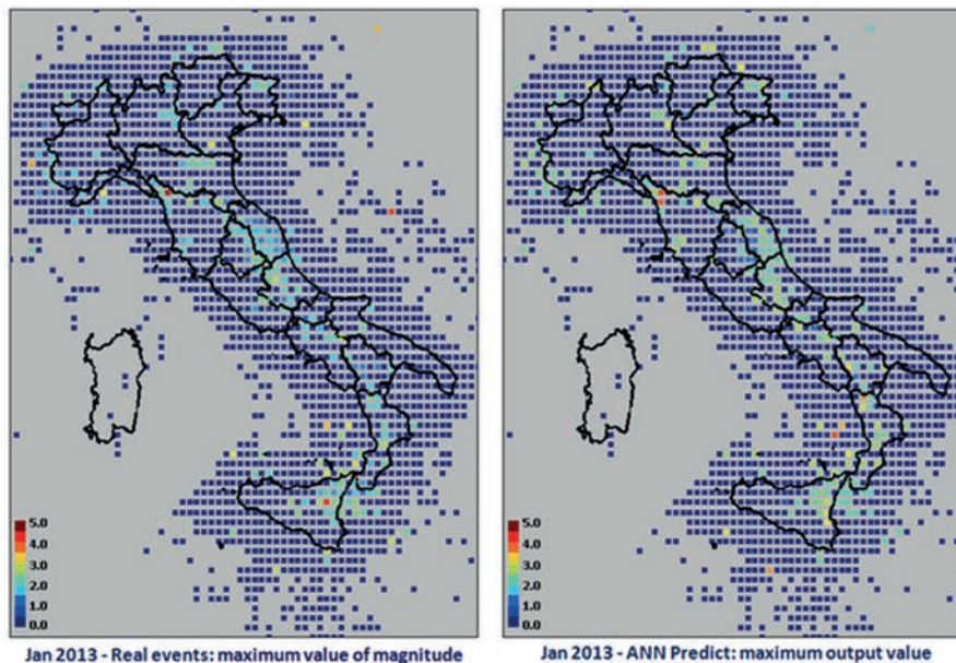
Fig. A7 - Results of January 2013: a) maximum magnitude of real events; b) maximum magnitude predicted by ANN.
