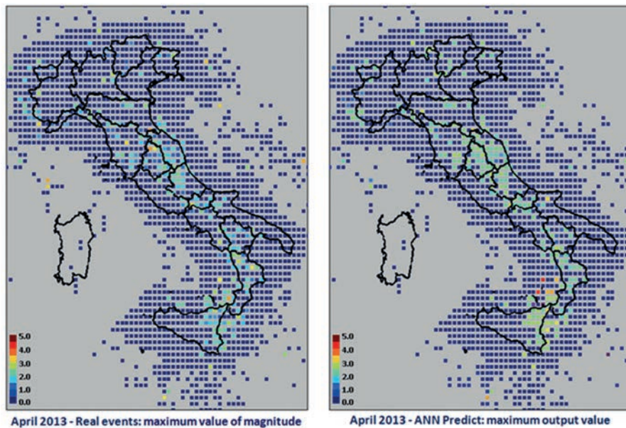
Fig. A10 - Results of April 2013: a) maximum magnitude of real events; b) maximum magnitude predicted by ANN.
