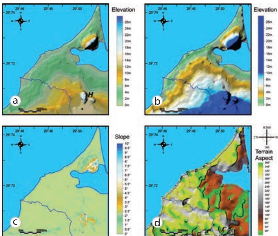
Fig. 3 - Topographic surface analyses obtained by processing 1:1000 data: a) DTM; b) DTM with a particular colour scale to enhance elevation differences. Despite small artefacts due to infrastructures and the not uniform original data sampling, the morphology of the delta lobes is evident; c) terrain slope; d) terrain aspect. The western portion of the plain has a mean slope direction towards NW, while the eastern part towards NE.
