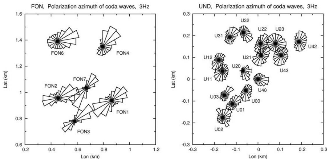
Fig. 7 - Distributions of polarization azimuth of coda waves (average among all earthquakes) computed for any stations of the two arrays at the central frequency of 3 Hz. At FON array a predominant NE-SW direction is seen at all stations.
