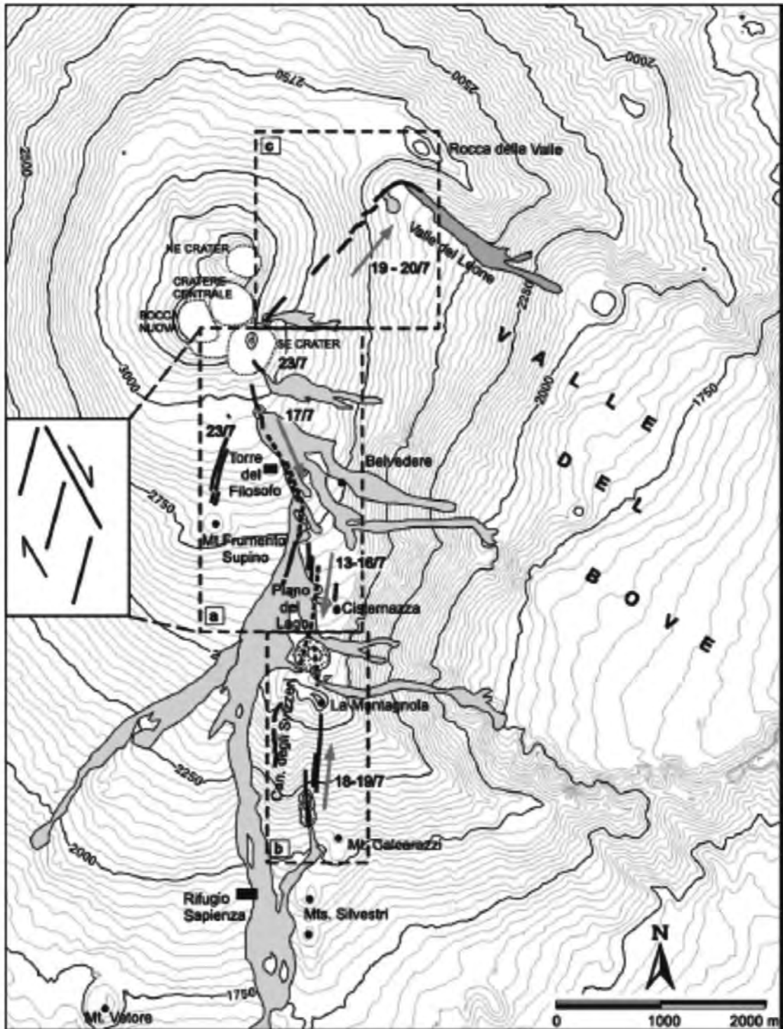
Fig. 3 - Map of the eruptive fracture systems and lava flows formed during the 2001 July 17-August 9 flank eruption. Three main fracture fields have been recognized on the basis of the time-space development of distinct segments: (a) Piano del Lago field; (b) Montagnola field; (c) Valle del Leone field. Gray arrows indicate the sense of migration of each fracture field (after Monaco et al. , 2005).
