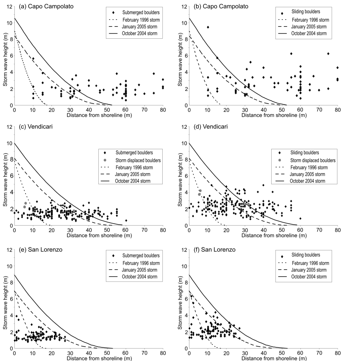
Fig. 7 - Flooding landward limit of the strongest storm waves at: Capo Campoloto site [(a) and (b)]; Vedicari site [(c) and (d)]; San Lorenzo site [(e) and (f)]; (storm breaking wave H_b and relative period are reported in Table 1). Black diamonds are the values of the storm wave heights when each boulder was deposited at its distance from the shoreline, computed by applying the flow transport mechanism (graphs on the left) and the sliding transport mechanism (graphs on the right) by Noormets et al. (2004). Grey dots are boulders emplaced by the 2009 winter storm waves at Vedicari.
