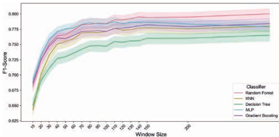
Fig. 8 - Effect of W on classification F1-score. This figure illustrates the variation in classification F1-score for different ML models as a function of sliding W . The shaded regions represent confidence intervals, highlighting the stability and generalisation of each model.
