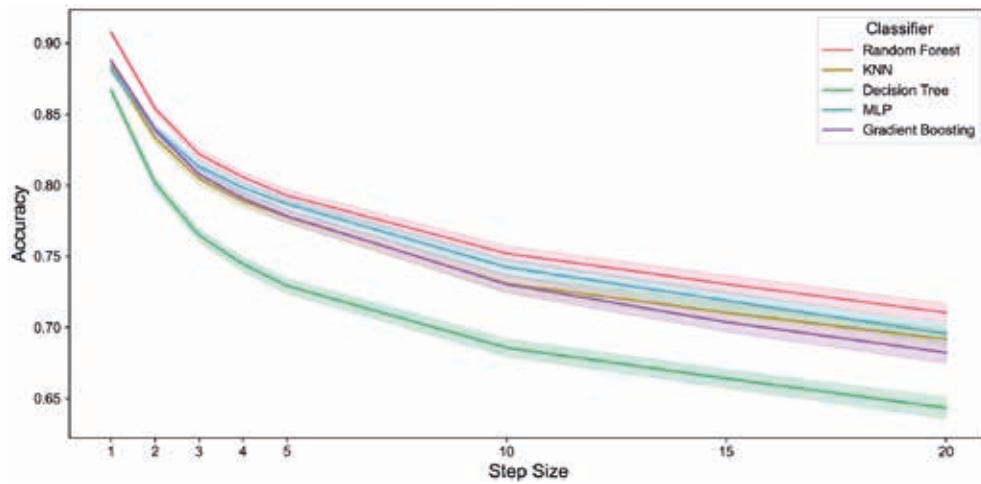
Fig. 10 - Effect of S on classification accuracy. This figure illustrates the variation in classification accuracy for different ML models as a function of S . The shaded regions represent confidence intervals, highlighting the stability and generalisation of each model.
