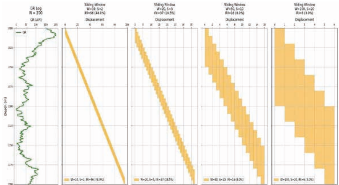
Fig. 3 - Effect of sliding window parameters on geophysical well-log segmentation and IRI . This figure illustrates the impact of varying sliding window configurations on the segmentation of GR well log ( N = 200 samples). The GR log is displayed on the left, followed by four panels showing displacement patterns resulting from different W and S combinations. Specifically, the configurations include W = 10 , S = 2 ( IRI = 96 ; IRI_{\%} = 48.0\% ), W = 20 , S = 5 ( IRI = 37 ; IRI_{\%} = 18.5\% ), W = 50 , S = 10 ( IRI = 6 ; IRI_{\%} = 3.0\% ), and W = 100 , S = 20 ( IRI = 4 ; IRI_{\%} = 1.0\% ). As the W increases and the S becomes coarser, the number of segments decreases and the overlap between windows reduces. This visualisation highlights how parameter choices influence data partitioning, which is critical for entropy-based analysis and ML-driven lithology classification.
