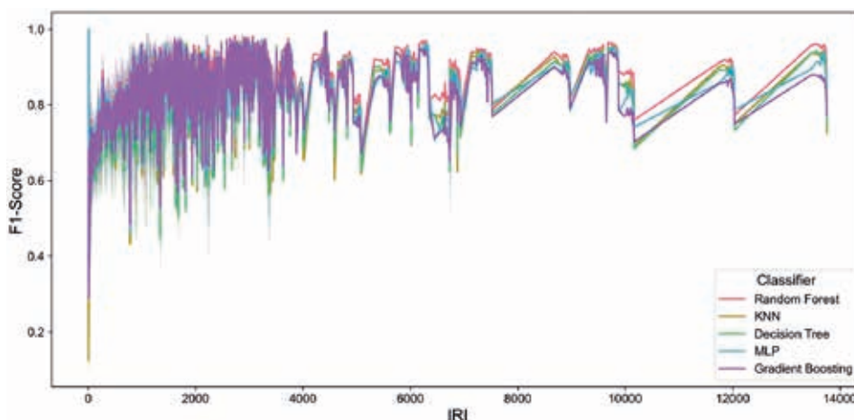
Fig. 16 - This figure illustrates the variation in the F1-score as a function of the IRI_{\%} : early fluctuations compress as the IRI grows, a transient mid-band dip appears, and performance plateaus near 0.9–1.0. RF remains the safest performer, with GB close behind.
