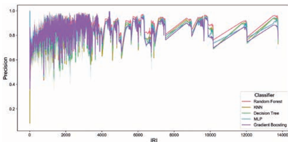
Fig. 15 - This figure illustrates the variation in precision as a function of the IRI_{\%} : large spread at low IRI values that tighten with greater IRI values, with a short boundary dip before stabilising at 0.9. RF and GB dominate; DT shows the widest early spread.
