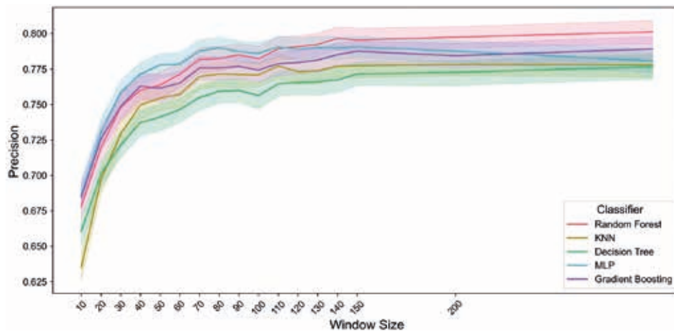
Fig. 7 - Effect of W on classification precision. This figure illustrates the variation in classification precision for different ML models as a function of sliding W . The shaded regions represent confidence intervals, highlighting the stability and generalisation of each model.
