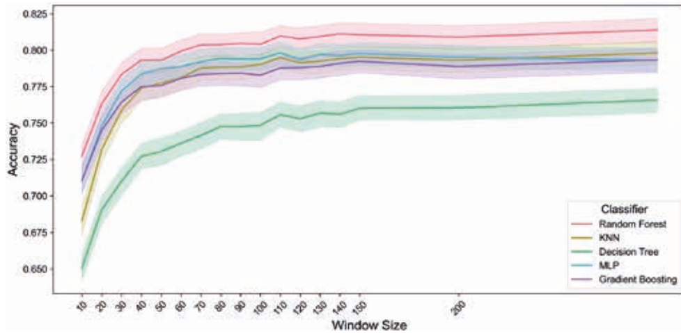
Fig. 6 - Effect of W on classification accuracy. This figure illustrates the variation in classification accuracy for different ML models as a function of sliding W . The shaded regions represent confidence intervals, highlighting the stability and generalisation of each model.
