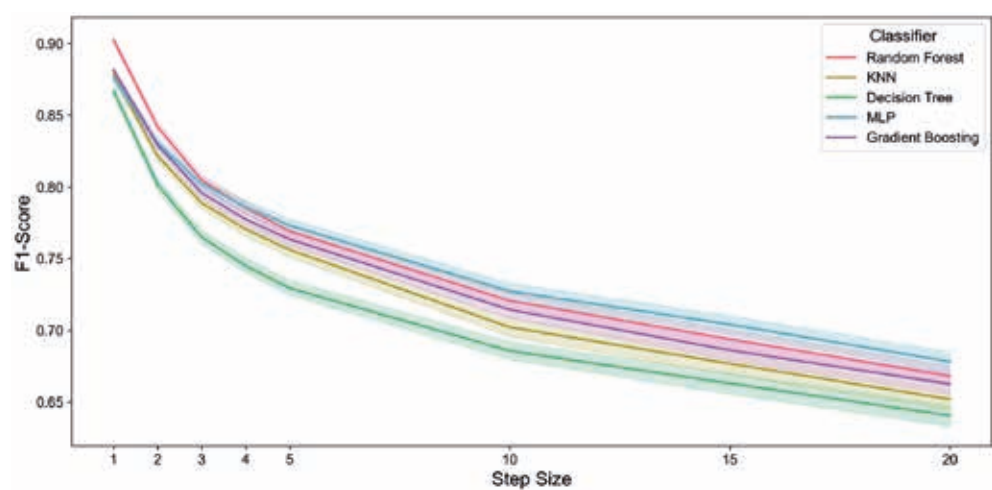
Fig. 12 - Effect of S on F1-score. This figure illustrates the variation in F1-score for different ML models as a function of S . The shaded regions represent confidence intervals, highlighting the stability and generalisation of each model.
