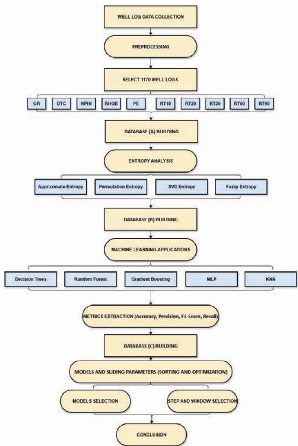
Fig. 2 - The adopted workflow for enhancing entropy-based lithology discrimination through sliding parameters. This figure illustrates the systematic workflow adopted in this study to optimise the sliding parameters, S and W , for improved lithology discrimination using entropy-based analysis. The methodology outlines a sequential approach, beginning with the collection of geophysical well-log data, followed by comprehensive data preprocessing, entropy computation, and the application of ML algorithms. The workflow is designed to fine-tune the sliding parameters, thereby maximising the effectiveness of entropy measures in distinguishing lithological variations.
