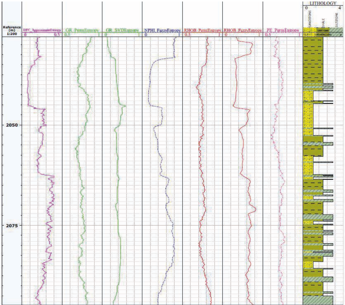
Fig. 4 - Example of entropy-based complexity profiles of some geophysical well logs. This figure presents entropy-based complexity profiles derived from geophysical well-log data, utilising four distinct entropy measures: ApEn , FuzzyEn , PermEn , and SVDEn . The analysis spans multiple geophysical logs, including GR, DTC, NPHI, and RHOB. The resulting profiles highlight subtle variations in signal complexity with depth, providing valuable insights into subsurface heterogeneity. The lithological classification is shown on the far right for correlation with the complexity profiles.
