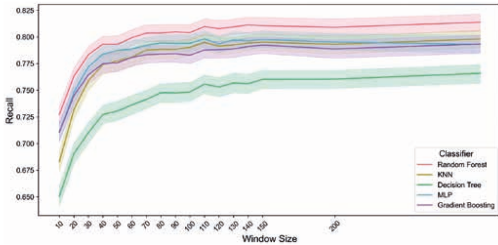
Fig. 9 - Effect of W on classification recall. This figure illustrates the variation in classification recall for different ML models as a function of sliding W . The shaded regions represent confidence intervals, highlighting the stability and generalisation of each model.
