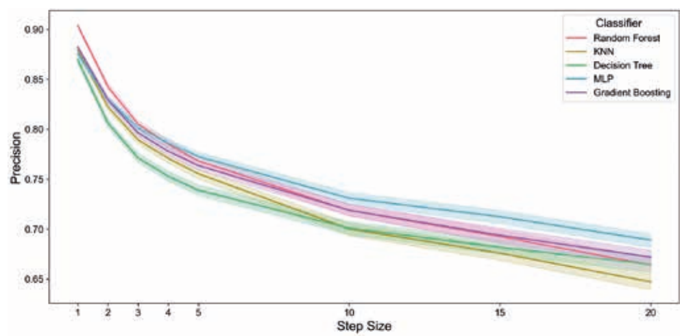
Fig. 11 - Effect of S on precision. This figure illustrates the variation in precision for different ML models as a function of S . The shaded regions represent confidence intervals, highlighting the stability and generalisation of each model.
