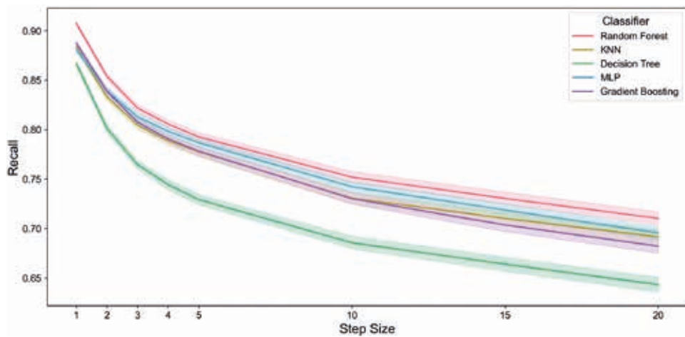
Fig. 13 - Effect of S on recall. This figure illustrates the variation in recall for different ML models as a function of S . The shaded regions represent confidence intervals, highlighting the stability and generalisation of each model.
