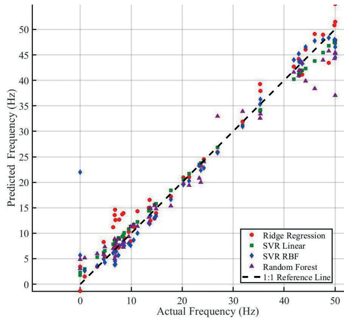
Fig. 4 - Actual versus predicted f_{\sigma} for the four models. Points clustered along the 1:1 reference line indicate good predictive alignment. RR and SVR RBF show the closest match to the ideal trend.
