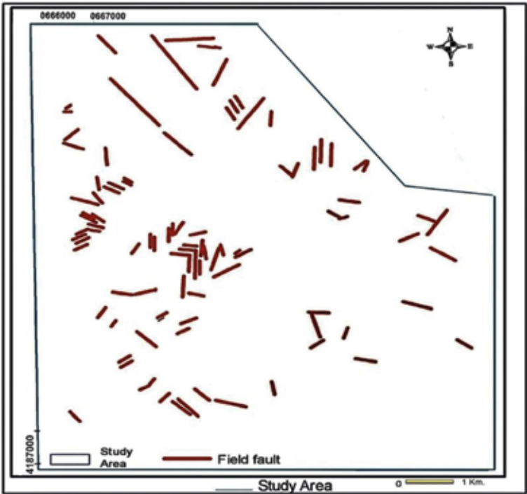
Fig. 9 - Fault map of the study area.
