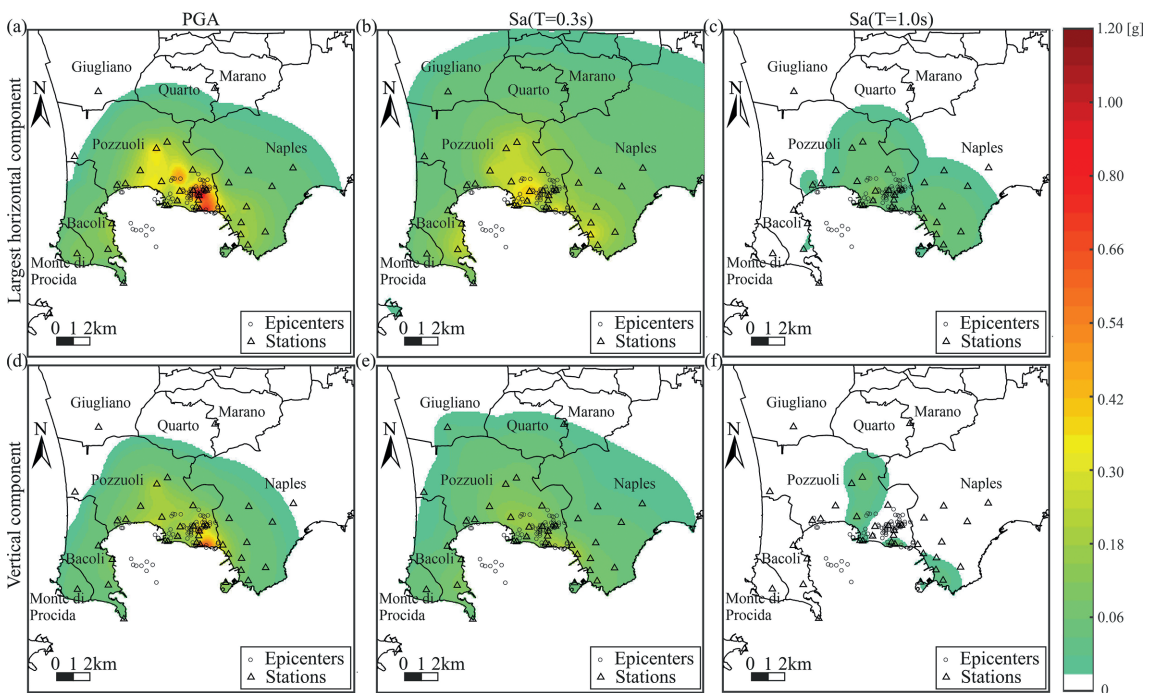
Fig. 6 - Maps of largest median shaking from the M_d \geq 2.5 events recorded from March 2022 to September 2025, in terms of PGA , Sa(T=0.3s) , and Sa(T=1.0s) . Considered events are those whose records are made available by RAN or ING.V. Panels a to c and panels d to f refer to the largest horizontal and vertical ground motion components, respectively.
