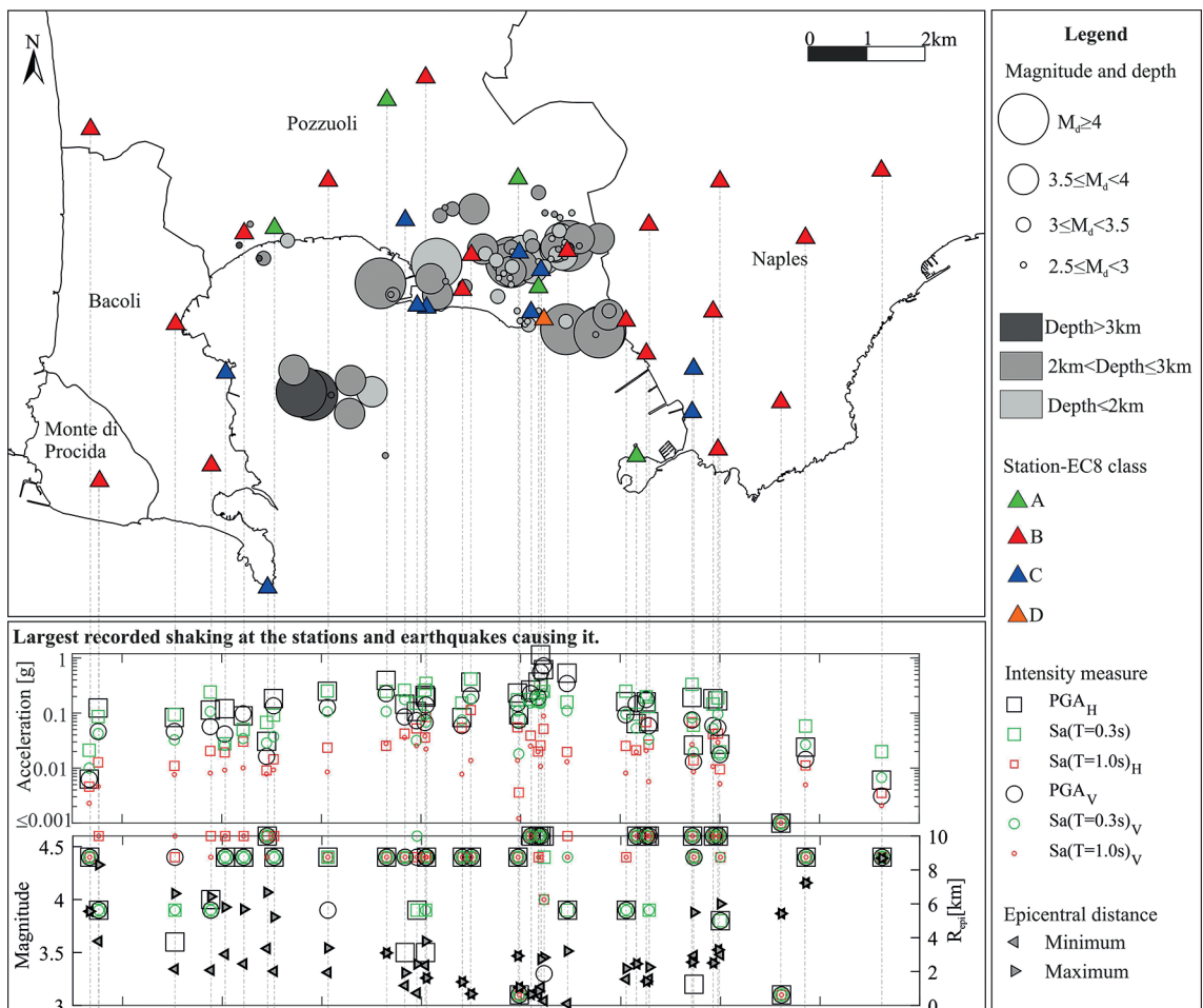
Fig. 2 - Epicentre, M_d , and depth of the M_d \geq 2.5 earthquakes recorded from March 2022 to September 2025, whose records are made available by RAN or ING V at the stations in the map. Below the map: the largest horizontal and vertical PGA , Sa(T = 0.3\text{ s}) , and Sa(T = 1.0\text{ s}) recorded and the corresponding earthquakes in terms of M_d and minimum and maximum R_{epi} .
