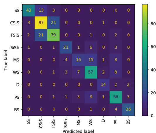
Fig. 5 - Confusion matrix of the FFNN model.
