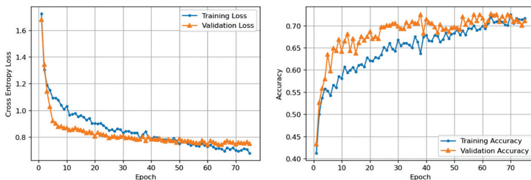
Fig. 6 - Training and validation curves for the FFNN model: a) loss and b) accuracy across epochs.
