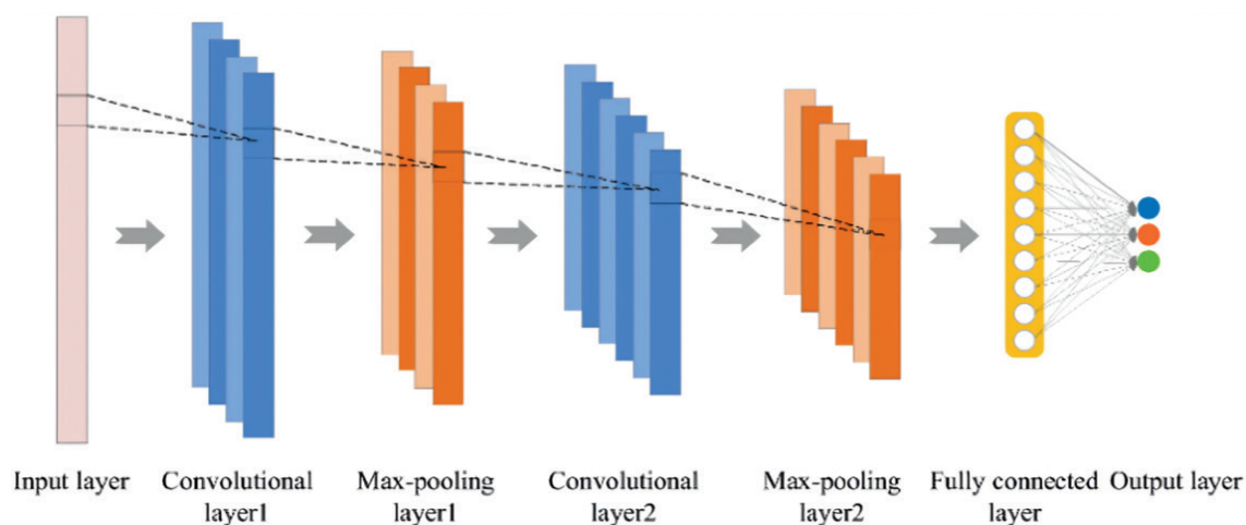
Fig. 1 - The structure of the 1D CNN model (Yang, 2022).
