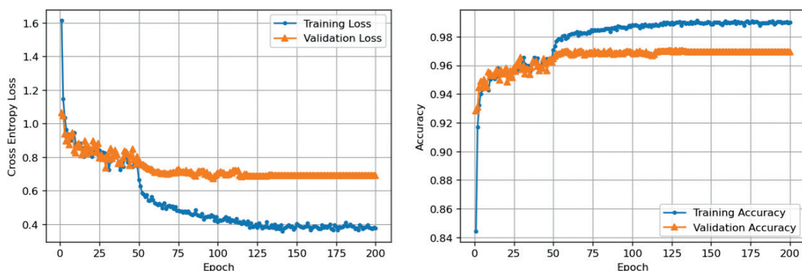
Fig. 2 - Training and validation curves for the CNN model: a) loss and b) accuracy across epochs.
