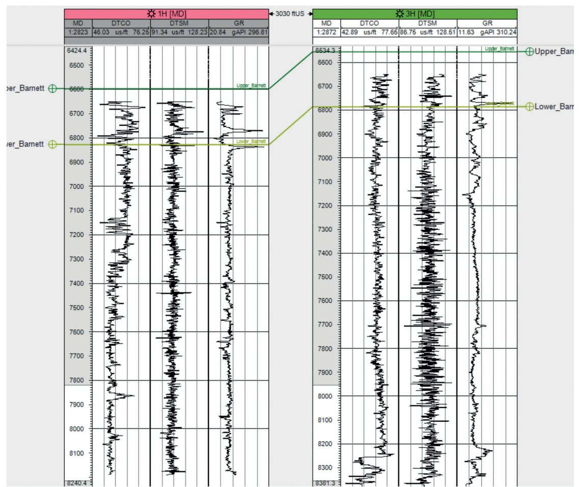
Fig. 3 - Raw well-log data used as input of the implemented MLP machine; track 1: measured depth, track 2: P-wave slowness, track 3: S-wave slowness, and track 4: natural gamma ray.
