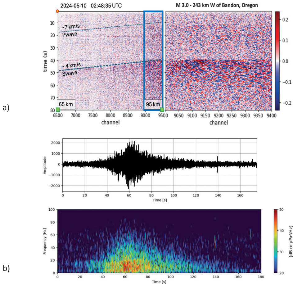
Fig. 3 - 10 May 2024 (02:48:35 UTC) earthquake: a) P- and S-seismic wave arrivals recorded by the optic fibre; b) waveform and spectrogram recordings from the southern hydrate hydrophone (window = hann, nfft = 8192, 25% overlap, sampling rate = 200 Hz).
