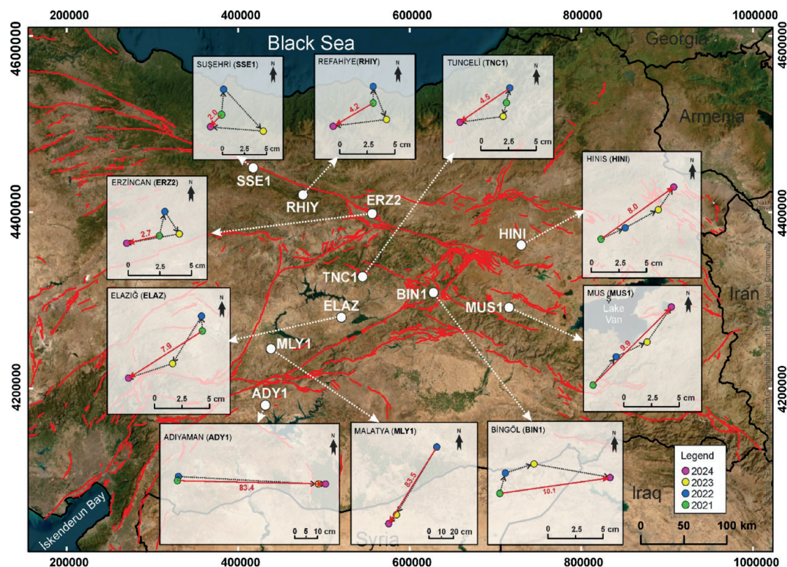
Fig. 6 - Map of the observed GNSS stations and horizontal velocities between 2021 and 2024.
