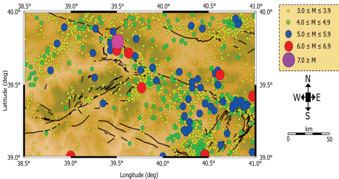
Fig. 2 - Epicentre locations of 2662 earthquakes with M_w \geq 3.0 from 1 Jan 1900 to 1 Mar 2024 for the study region. The seismicity catalogue is obtained from the KOERI (2024) website. Magnitude levels of the events are shown with circles of different colors and sizes.
