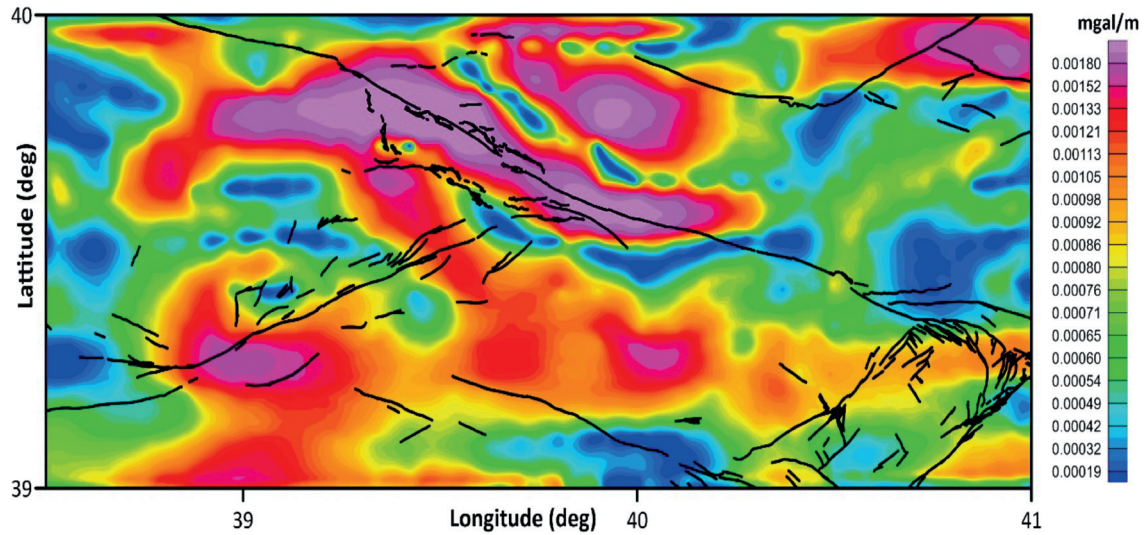
Fig. 4 - THD map of the study area.
