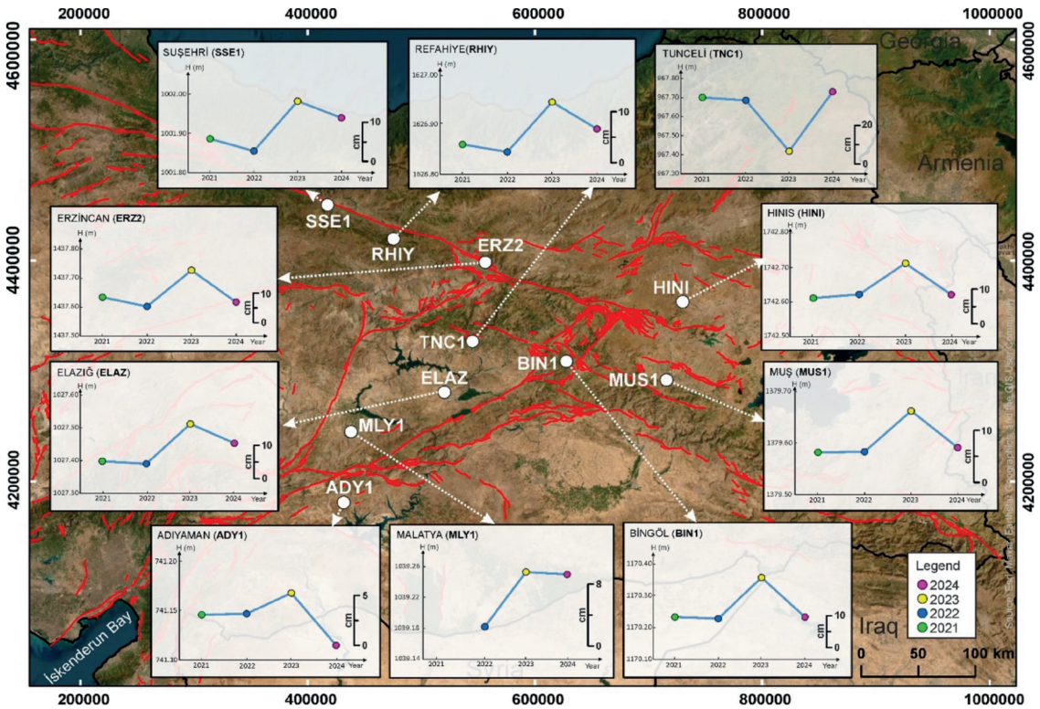
Fig. 7 - Map of the observed GNSS stations and vertical velocities between 2021 and 2024.
