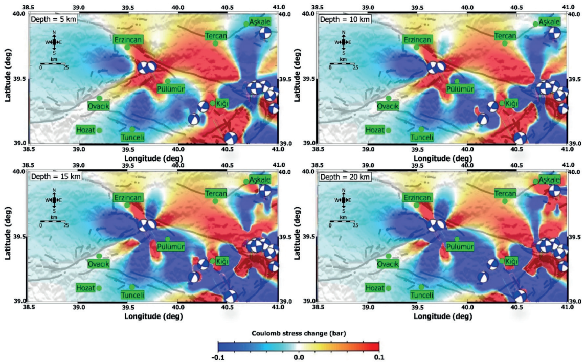
Fig. 8 - Coulomb stress changes (in bars) generated by earthquakes with a magnitude greater than M_w \geq 5.0 at depths of 5, 10, 15, and 20 km for the 2003-2023 period (for details see Table 5). Focal mechanism solutions represented by blue beach balls were taken from the GCMT (2024) and USGS (2024) websites. The black lines indicate the active faults in the study region modified by Emre et al. (2018). The green circles indicate the city locations. All calculations assumed an effective coefficient of friction ( \mu ) of 0.4 in harmony with the strike-slip fault mechanism.
