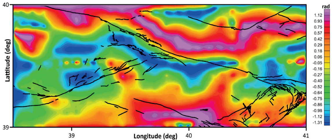
Fig. 5 - TA map of the study region.
