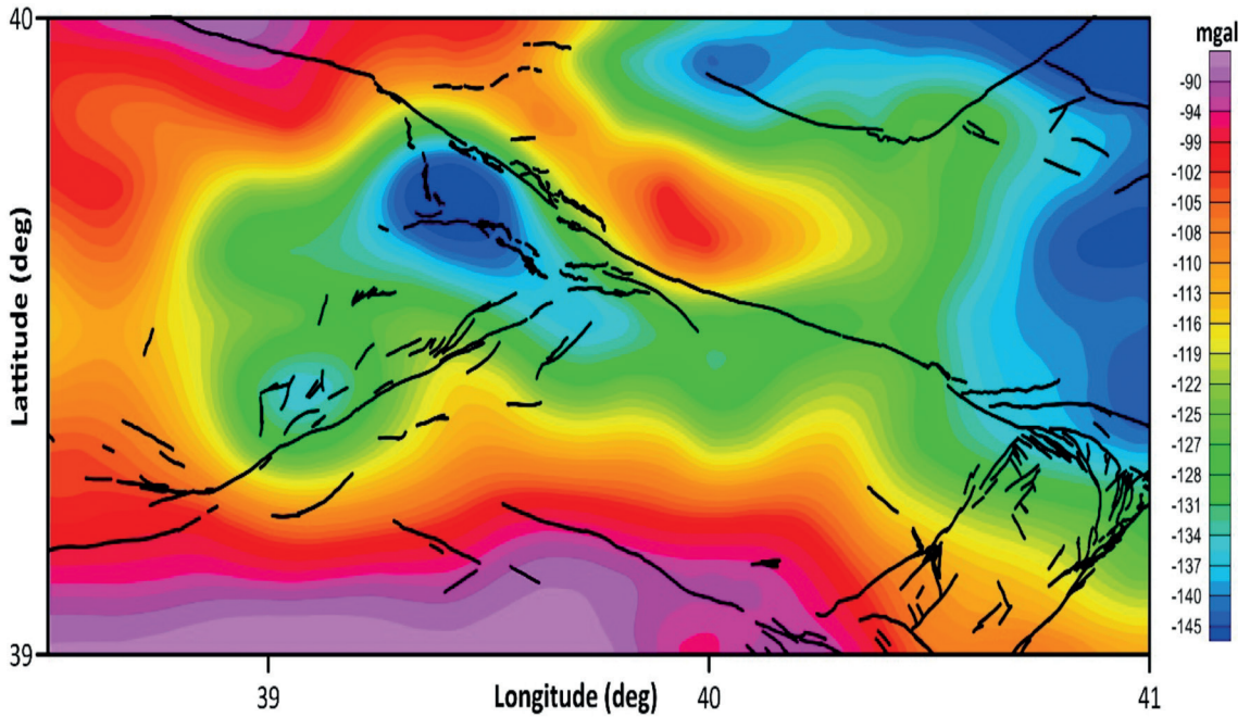
Fig. 3 - Gravity anomaly map of the study region. The gravity data with 10-kilometre gridded and active fault lines were obtained from MTA.
