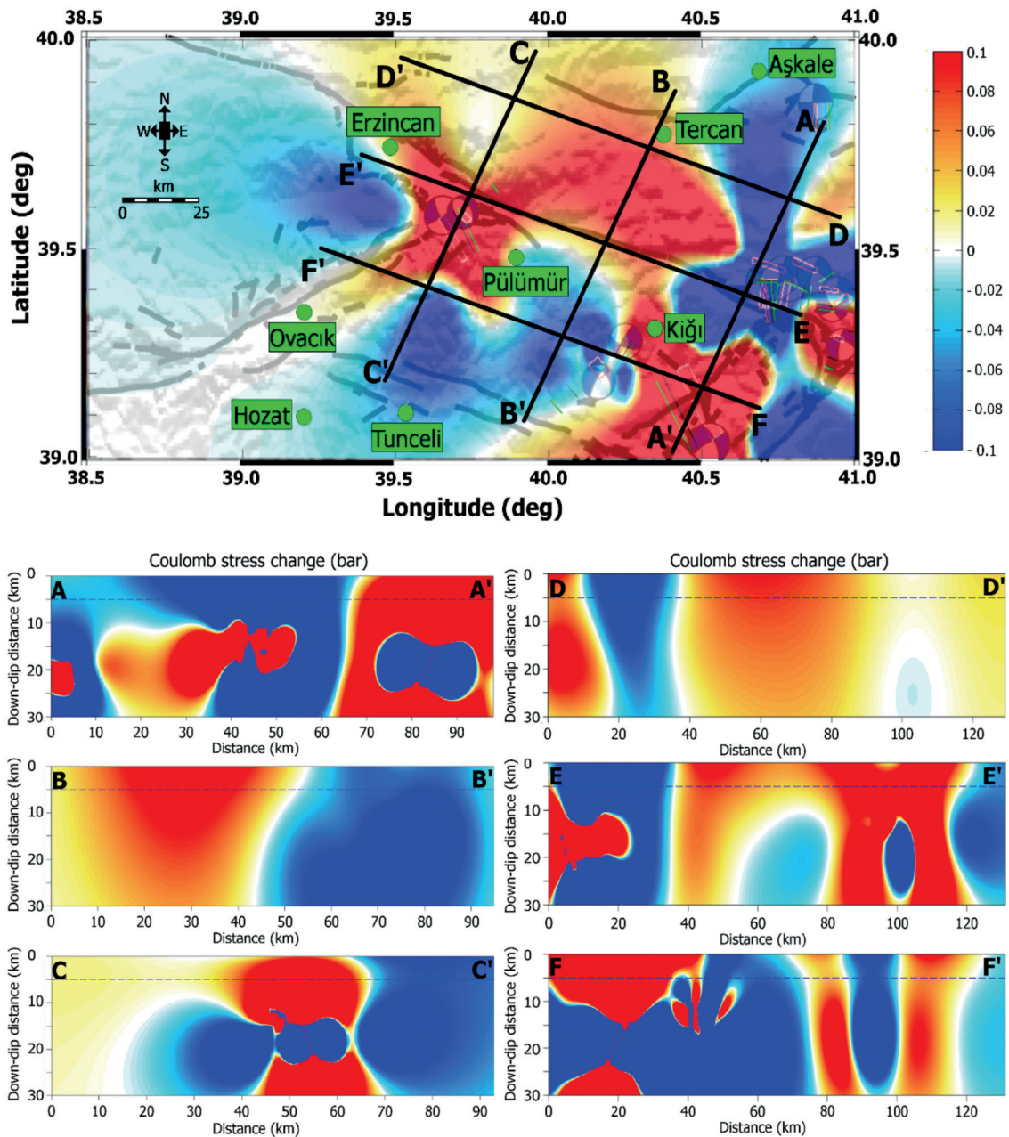
Fig. 9 - NE-SW (A-A', B-B', C-C') and NW-SE (D-D', E-E', F-F') oriented Coulomb stress cross-section profiles from 0 to 30 km, created from focal mechanism solutions shown in Fig. 8. The positive lobes are depicted in red and the negative lobes in blue.
