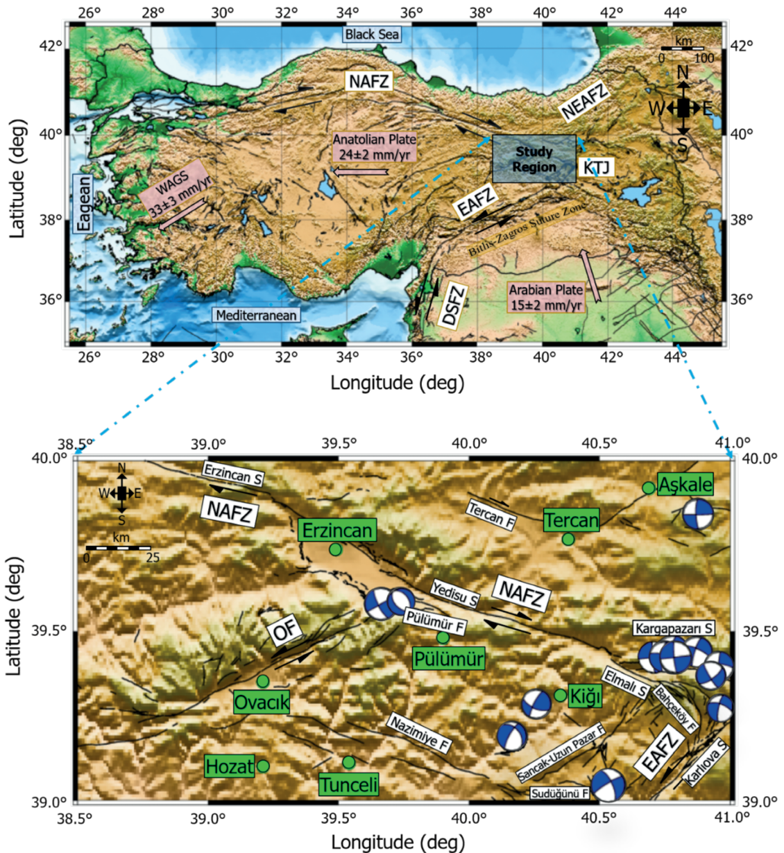
Fig. 1 - Top) Location of the study region with the main tectonic elements in and around the Anatolian region (modified from Emre et al. , 2018; Alkan et al. , 2023; Büyüksaraç et al. , 2024). The blue rectangle represents the study region. The pink arrows show the direction of plate motions with velocities (modified from Reilinger et al. , 2006). Bottom) Focal mechanism solution distributions of the earthquakes with M_L \geq 5.0 between 2003 and 2021 that occurred in the study region. The black arrows represent the direction of movement of fault and fault zones (taken from Emre et al. , 2018). The green circles represent the province locations. Abbreviations: NAFZ = North Anatolian Fault Zone, NEAFZ = NE Anatolian Fault Zone, EAFZ = East Anatolian Fault Zone, DSFZ = Dead Sea Fault Zone, KTJ = Karlıova Triple Junction, WAGS = West Anatolian Graben System, OF = Ovacık Fault, S = segment, F = fault.
