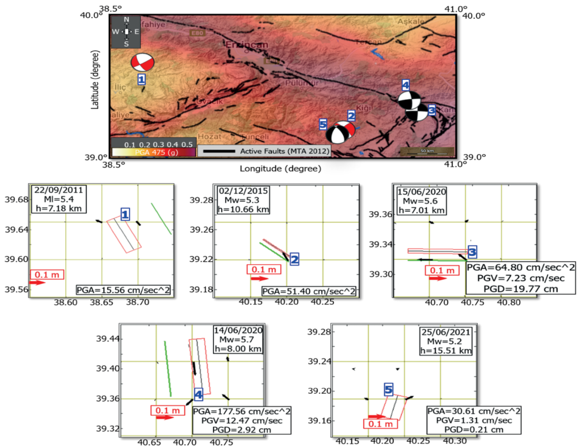
Fig. 10 - Horizontal displacement vector analyses for five local earthquakes with magnitudes greater than M \geq 5.0 in the study region. Black lines depict active fault zones taken from Emre et al. (2013). Catalogue information, PGA , PGV , and PGD values (the 1 st and 2 nd earthquakes have no PGV and PGD information), and focal mechanism solutions of earthquakes are shown in the centre of the figure taken from the AFAD (2024) website. Five small rectangles indicate the horizontal displacement vectors. The black arrows depict the displacement of each earthquake. These figures were obtained from the Coulomb 3.4 software and modified with Zabcı et al. (2017).
