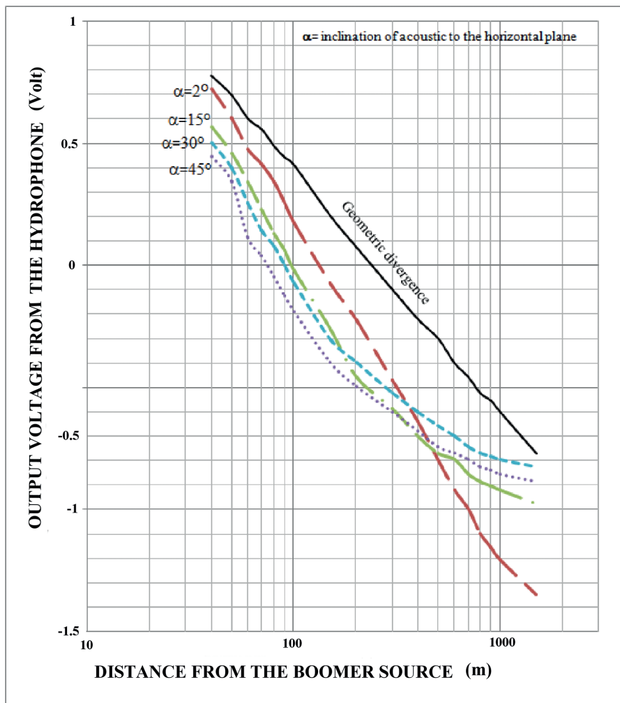
Fig. 13 - Attenuation of the sound pulse in different directions of a vertical plane passing through the generator. \alpha is the angle of the direction of propagation with the horizontal plane.
