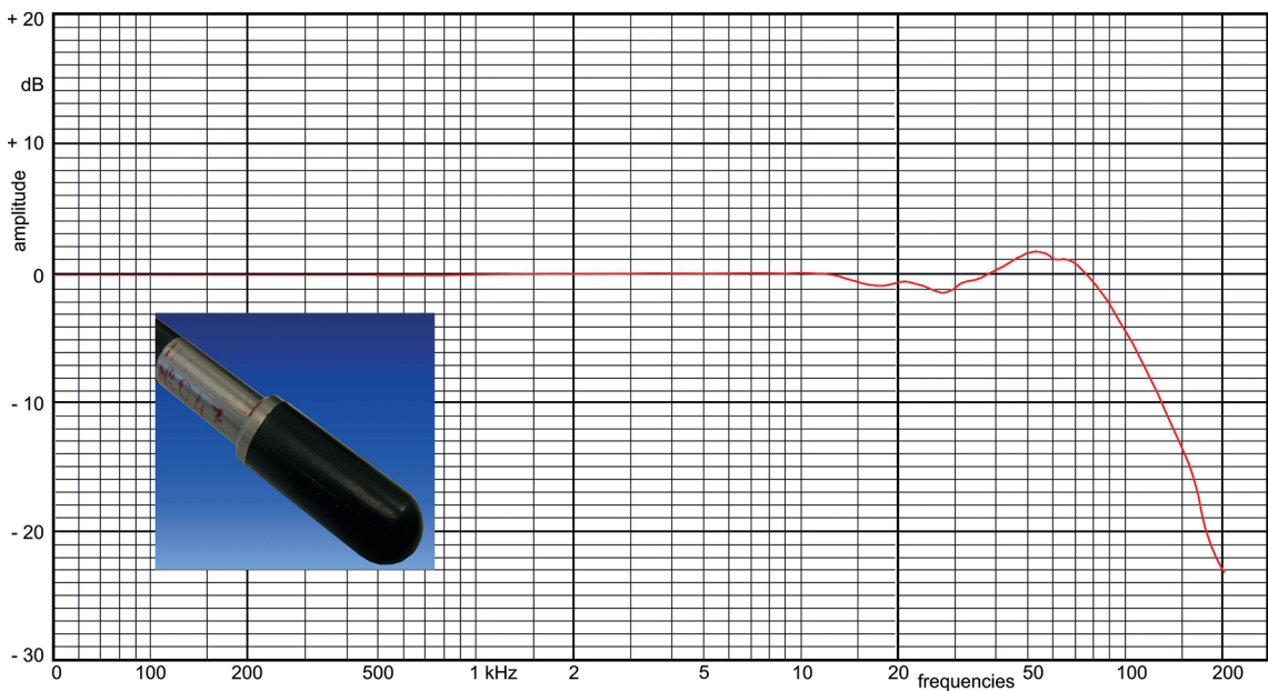
Fig. 2 - Bruel & Kier reference hydrophone.
