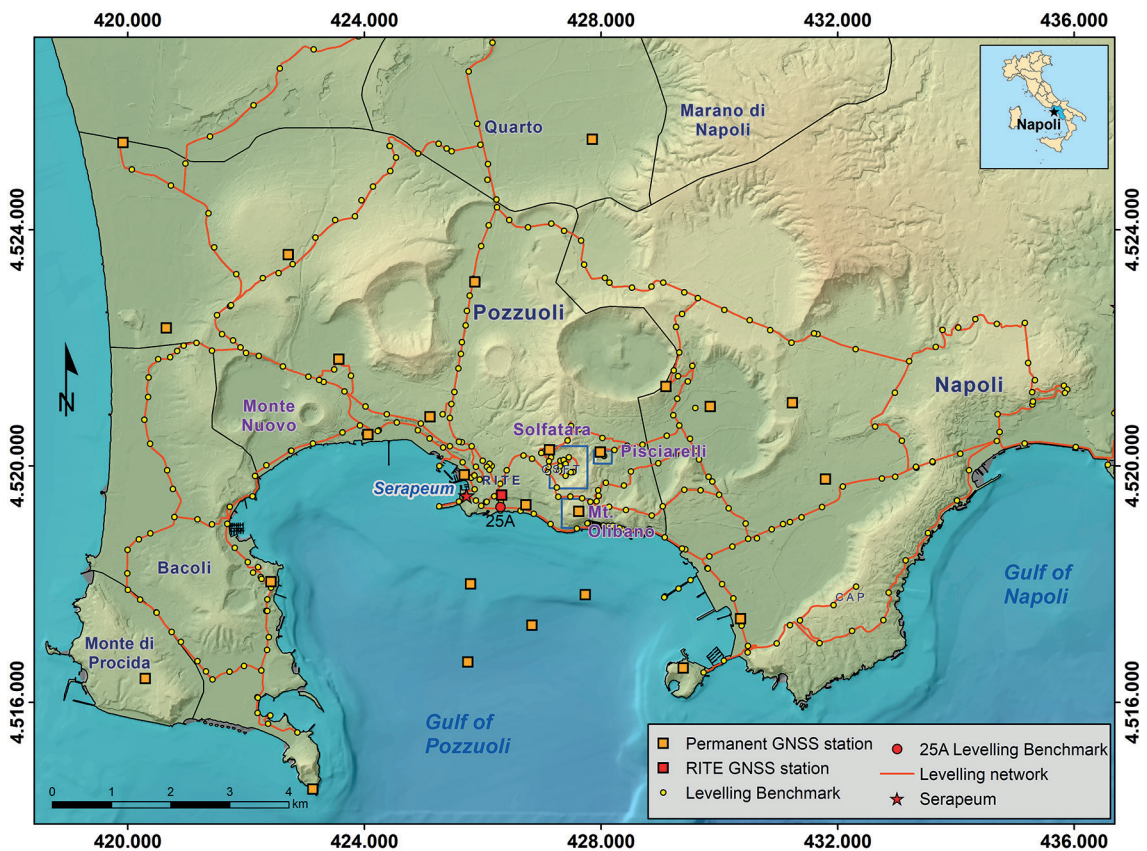
Fig. 1 - Map showing the Campi Flegrei area. The upper right insert reports the location of the area inside the Italian territory. The Digital Terrain Model (DTM) of Campi Flegrei is in UTM WGS84 (Vilardo et al. , 2013). The blue squares highlight the Solfatara crater, Pisciarelli area, and Mount Olibano. The Global Navigation Satellite System (GNSS) stations, levelling network, and benchmark are indicated according to the legend on the bottom right.
