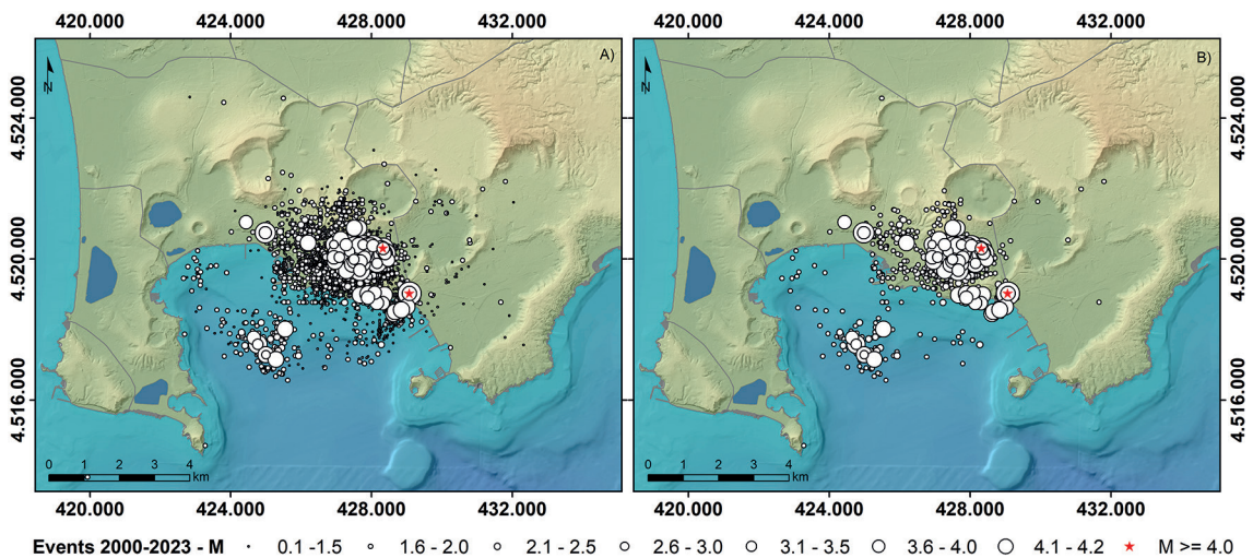
Fig. 7 - Spatial distribution of the seismicity, which occurred between January 2000 and December 2023 [from the OV-INGV catalogue ( https://terremoti.ov.ingv.it/gossip/flegrei/ )]: A) all located seismic events; B) seismic events with M \geq 1.5 . Circles are proportional to the magnitude of the events (see legend at the bottom). The stars represent the epicentres of the two M \geq 4 events.
