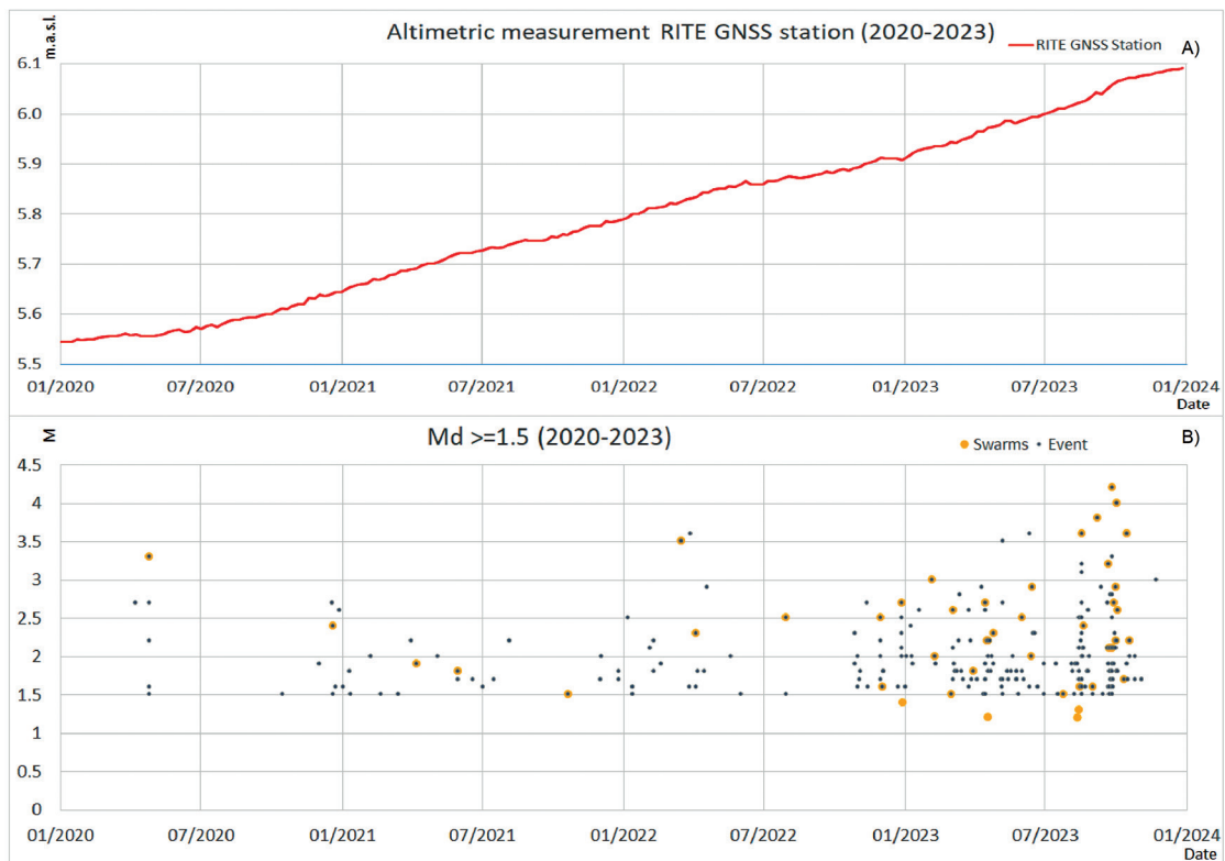
Fig. 8 – A) Altimetric profile at the RITE GNSS station between January 2020 and December 2023. B) Seismic activity with M \geq 1.5 occurred in the same time period. The yellow circles represent the seismic swarms, which occurred.
