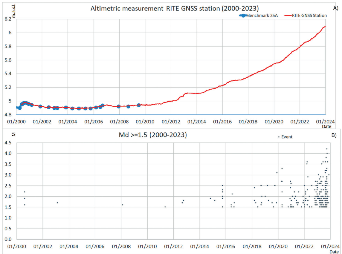
Fig. 6 – A) Altimetric profile at the RITE GNSS station between January 2000 and December 2023 (red line). The blue dots represent the altimetric profile obtained from the geodetic levelling surveys at benchmark 25A until 2009. B) Seismic activity with M \geq 1.5 between January 2000 and December 2023.
