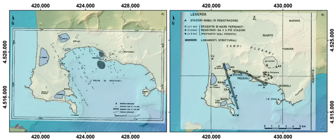
Fig. 3 - Spatial distribution of the located seismicity, which occurred during the 1969-1972 unrest [redraw after: A) Guerra et al. (1972) and B) Rampoldi (1972)]. The original figures were scanned and georeferenced in UTM WGS84 to make them compatible with the detailed cartographic bases used in this study. Legend Fig. 3A: triangles = seismic stations; dots = epicentres with h > 1.2 km; dashed area = epicentres with h < 0.5 ; dashed line = hypothesise fault. Legend Fig. 3B: triangles = temporary seismic stations; dots = epicentres of micro earthquakes acquired from three or more stations (depth of the hypocentres: empty dot < 1 km; half-full 1-3 km; full dot > 3 km); line = structural line.
