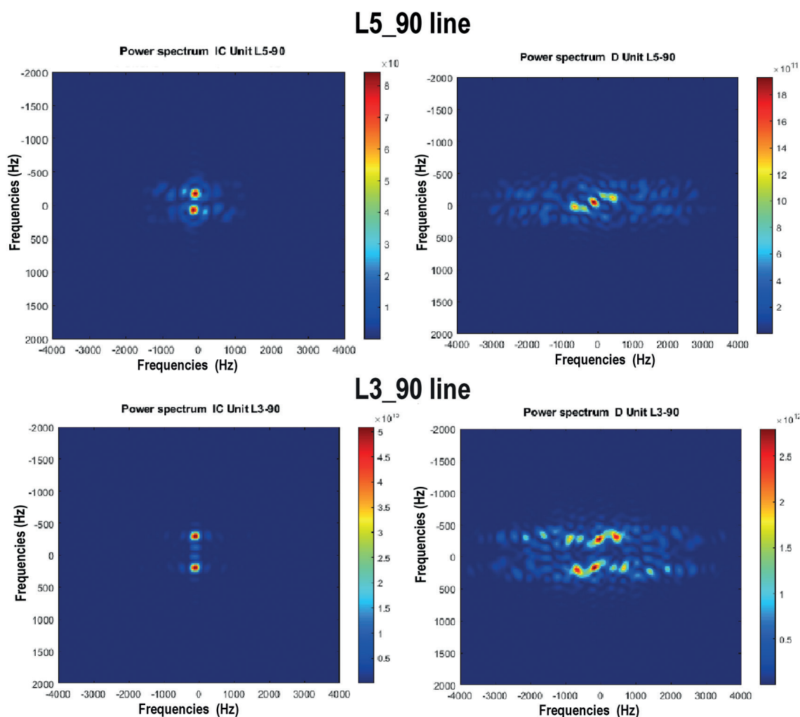
Fig. 11- Power spectrum: comparison between unit IC and unit D. Images are slightly zoomed for better reading.
