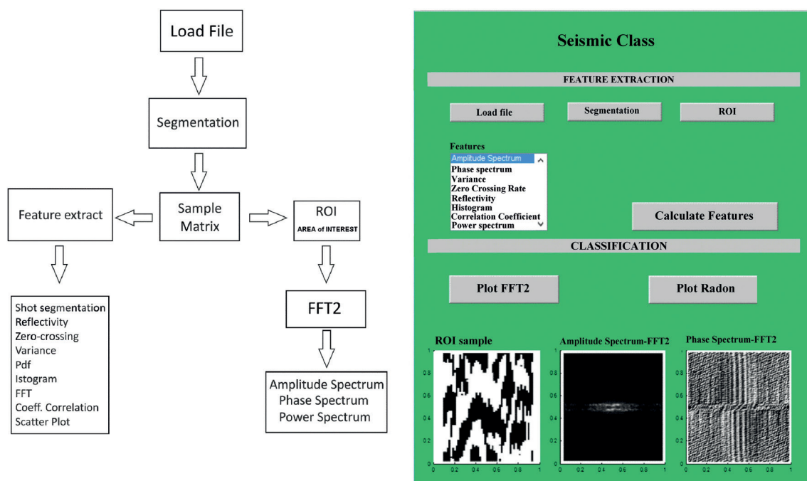
Fig. 1 - Main screen of the Seismic CLASS toolbox and relative block diagram.
