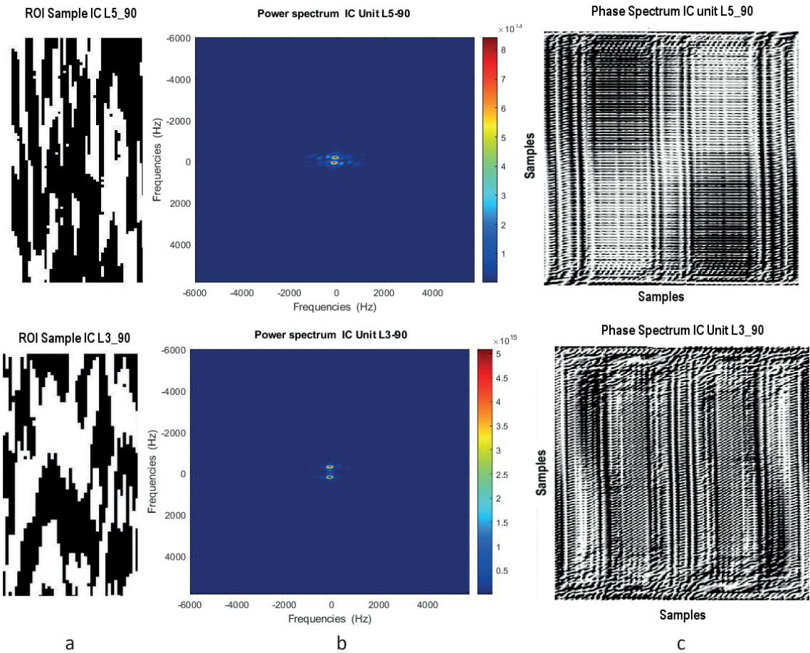
Fig. 7 - IC unit (L5_90 line-L3_90 line): a) ROI sample; b) amplitude spectrum response, FFT2.; c) phase spectrum response.
