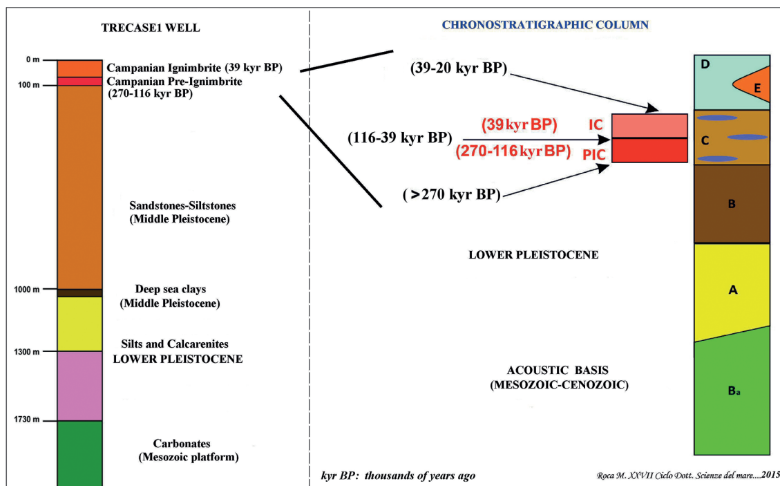
Fig. 2 -Stratigraphy of the Trecase1 well (Milia et al. , 2003; Milia and Torrente, 2011).
