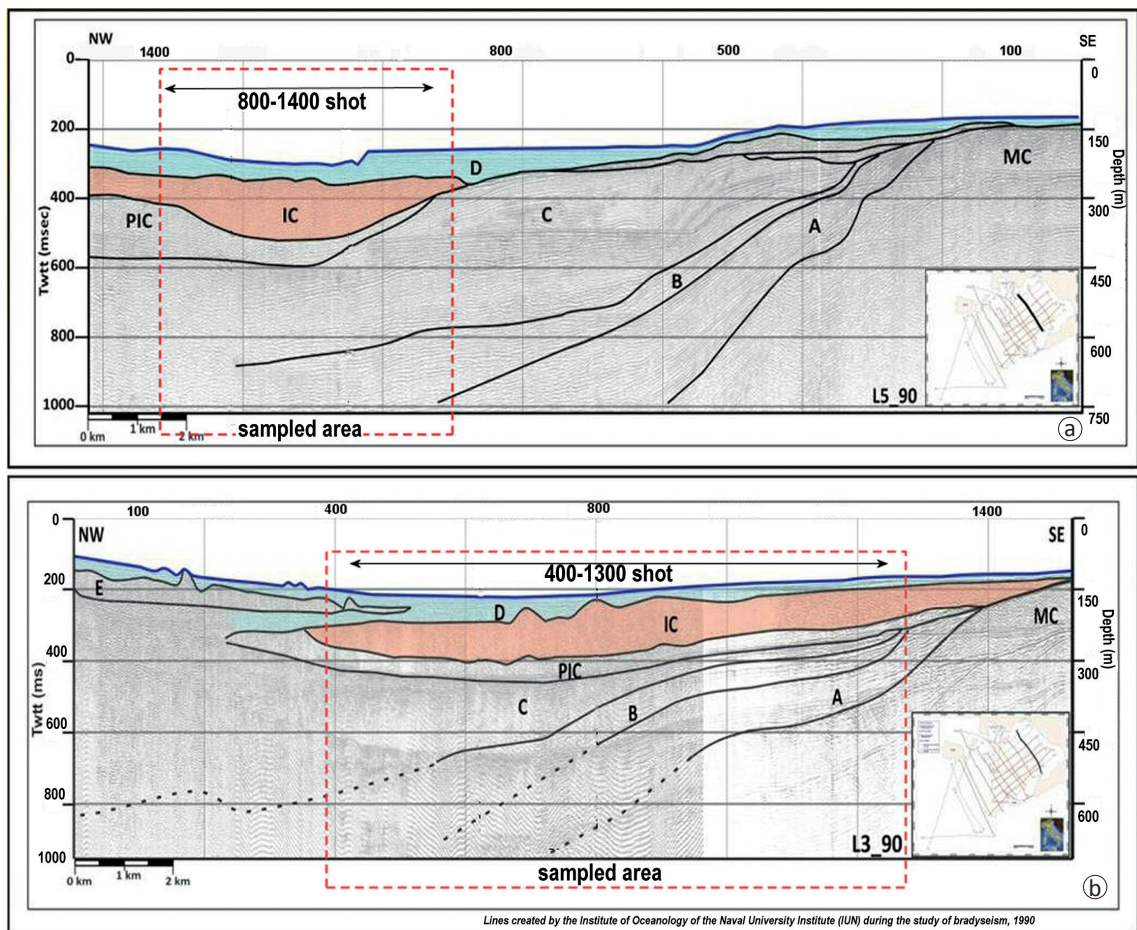
Fig. 5 - Seismic line interpretation: a) L5_90, b) L3_90. D unit = upper Pleistocene-Holocene marine sediments (39 kyr BP); IC unit = Campanian ignimbrite (39 kyr B.P.); PIC unit = pre-Campanian ignimbrite tuffs (270-116 kyr B.P.); C unit = middle-upper Pleistocene marine sediments; B unit = lower-middle Pleistocene marine sediments; A unit = upper Pliocene-lower Pleistocene marine sediments; MC unit = meso-Cenozoic carbonate bedrock (acoustic basement).
