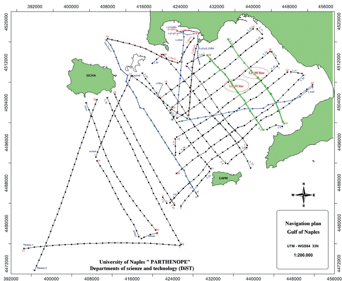
Fig. 3 - Navigation plan of the Gulf of Naples: the lines used are bold green.
