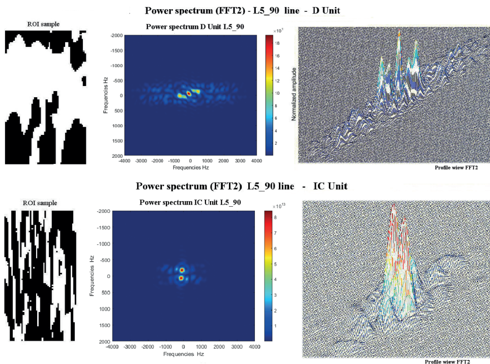
Fig. 9 - Picture sample and relative amplitude spectrum, line L5_90: a) D unit; b) IC unit.
