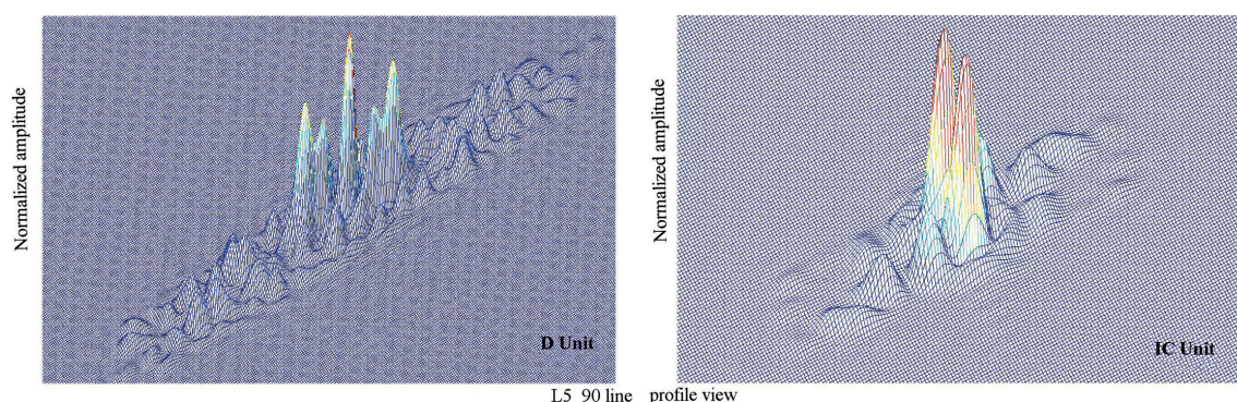
Fig. 10 - Comparison of the amplitude spectrum of the D unit and IC unit, L5_90 line (the spectra are slightly tilted for better viewing).
