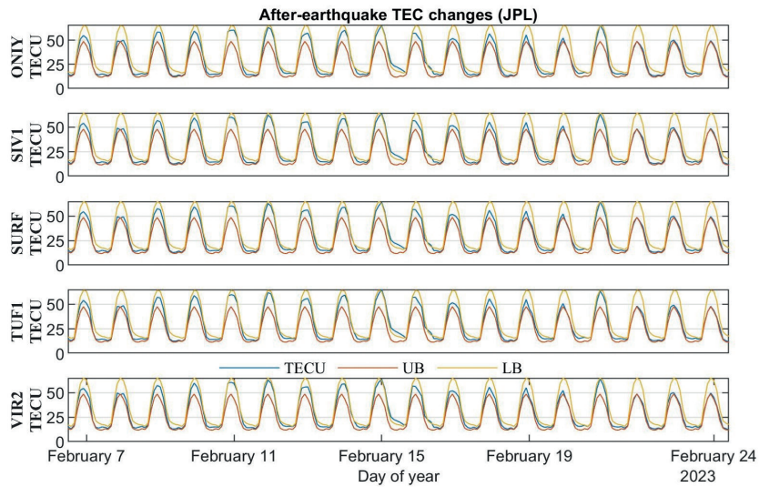
Fig. 21 - TEC, UB, and LB for the ONiy, SIV1, SURF, TUF1, and VIR2 stations from 7 to 24 February 2023.
