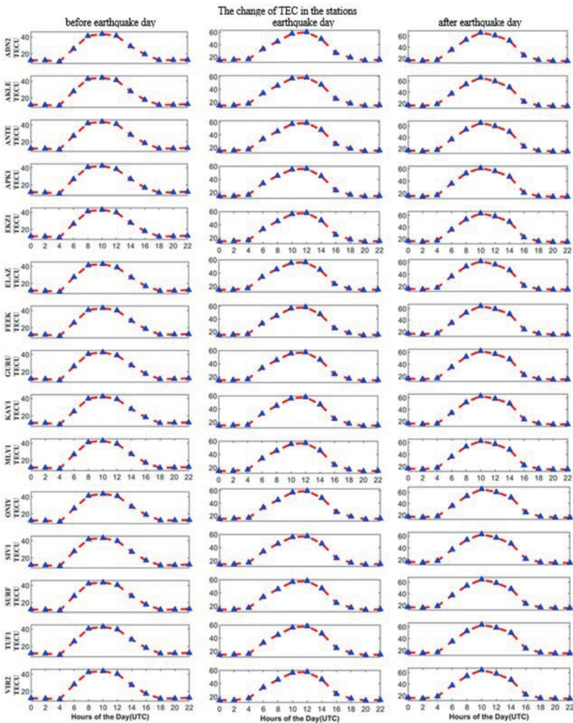
Fig. 16 - The change of TEC in the stations which are located at the earthquake area at before/during/after earthquake.
