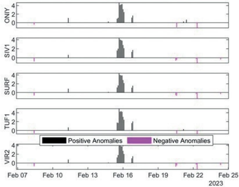
Fig 22 - The anomaly days for the ONiy, SIV1, SURF, TUF1, and VIR2 stations (TECU) from 7 to 24 February 2023.
