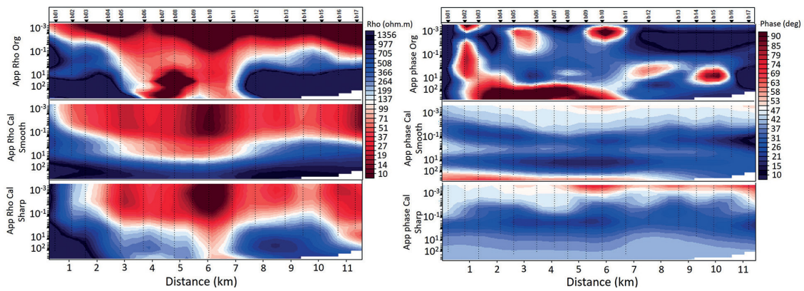
Fig. 15 - TE mode from MT data along profile B over the Mahallat geothermal reservoir including observed and calculated sections. A bimodal data inversion was executed (TE+TM).
