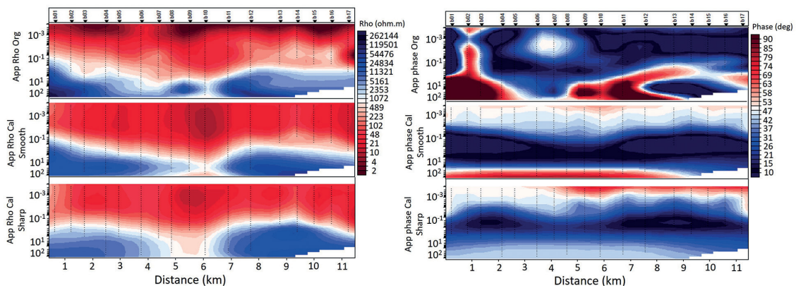
Fig. 16 - TM mode from MT data along profile B over the Mahallat geothermal reservoir including observed and calculated sections. A bimodal data inversion was executed (TE+TM).
