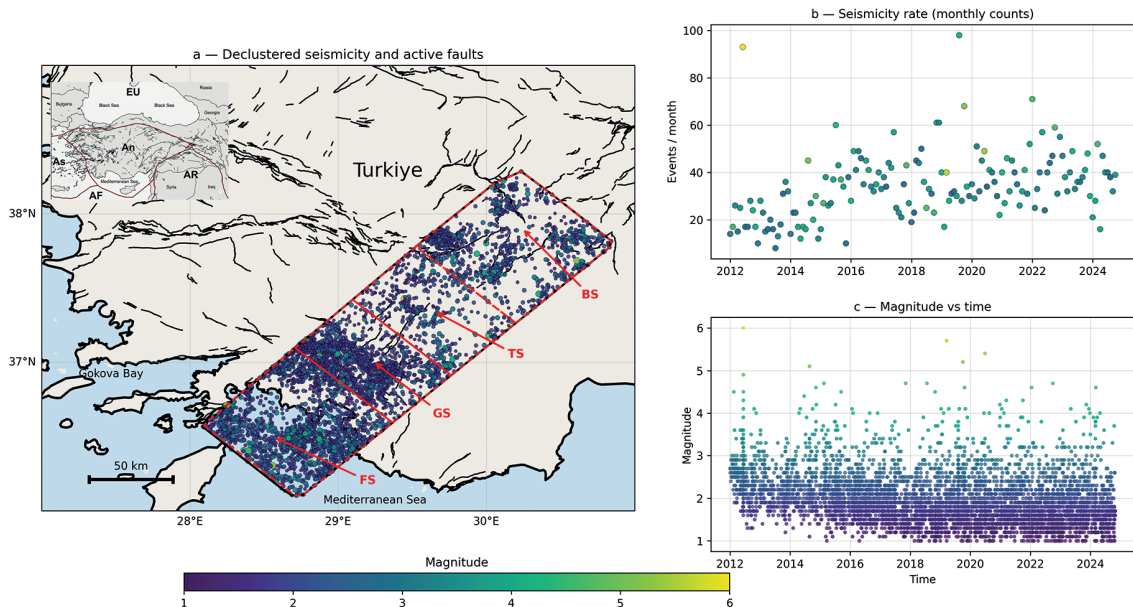
Fig. 1 - a) Decustered earthquake catalogue [ M_L \geq 1.0 earthquakes that occurred between 2 January 2012 and 31 December 2024 (KOERI, 2025)] and active faults within the study area. Earthquakes located inside the analysis polygon (red outline) are colour-coded according to magnitude. Black lines indicate fault segments [Fethiye segment (FS), Gölhisar segment (GS), Tefenni segment (TS), Burdur segment (BS)]. b) Monthly seismicity rate (number of events), point colours represent the maximum magnitude (max M ) observed in each month. c) Magnitude–time distribution for the same dataset. In all panels, the colour scale represents earthquake magnitude and a common colour scale is used across all panels. The inset map shows the plate boundaries in and around Turkey: African (AF), Arabian (AR), Eurasian (EU), Anatolian (An), and the Aegean sea (As) plates. The black thick lines represent fault lines (Şaroğlu et al. , 1992).
