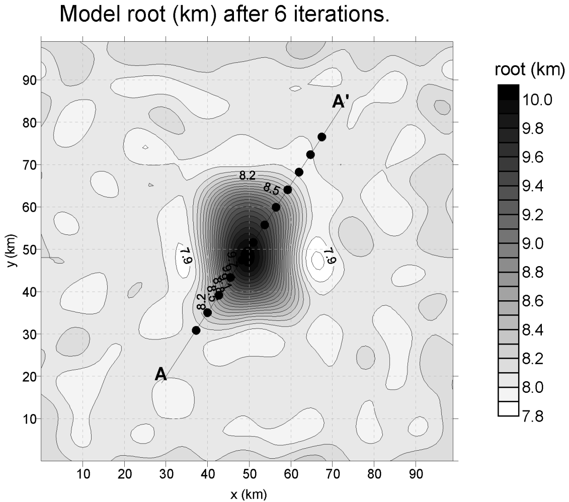
Fig. 4 - Map of the 3D inverted root after 6 iterations with position of constraining data (dots) and profile AA'.
