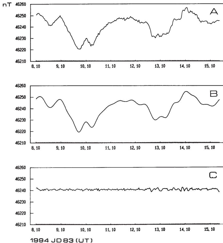
Fig. 4 - Total intensity F magnetograms of the geomagnetic field for the period 8 10 (UT): 15 32 (UT) - 1994JD83, recorded with a sampling rate of 2 min by the magnetometric station on the Isle of Tino (A); background geomagnetic signal: LP 1.4 \times 10^{-3} Hz (B); local artificial noise field: HP 1.4 \times 10^{-3} Hz (C).
