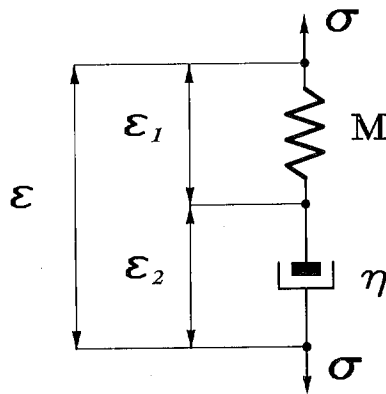
Fig. 3 — Mechanical model for a Maxwell substance. The force on both elements is the same but the elongation (strain) is different.
