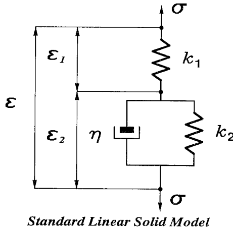
Fig. 13 — Standard linear solid mechanical model.
