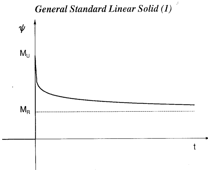
Fig. 23 — Relaxation function of the general standard linear solid composed of L elements connected in parallel (constant- Q model).
