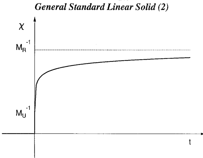
Fig. 24 — Creep function of the general standard linear solid composed of L elements connected in series (constant- Q model). The curve is very similar to the experimental creep function shown in Fig. 2.
