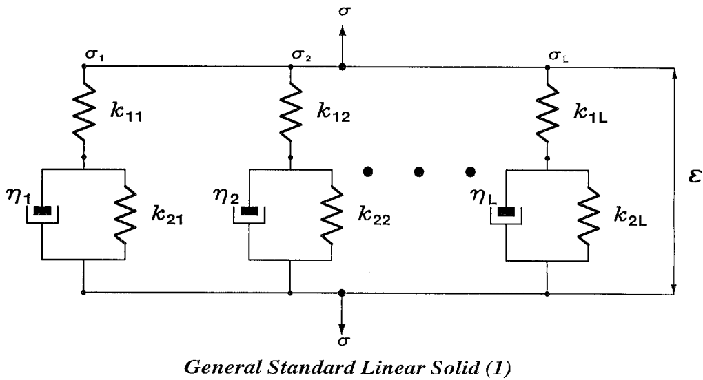
Fig. 19 — General standard linear solid model composed of L single elements connected in parallel. The same strain acts on each element.
