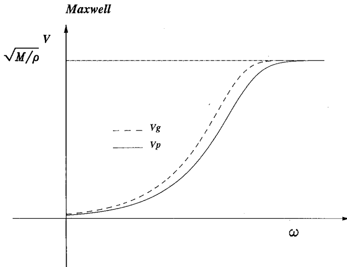
Fig. 5— Phase and group velocities of the Maxwell model. The elastic velocity is obtained at the high frequency limit. At the low frequency limit there is no propagation.
