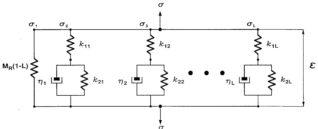
Fig. 18 — Liu et al.'s mechanical model has a spring with negative constant of value M_R(1-L) , where L is the number of standard linear solid elements.
