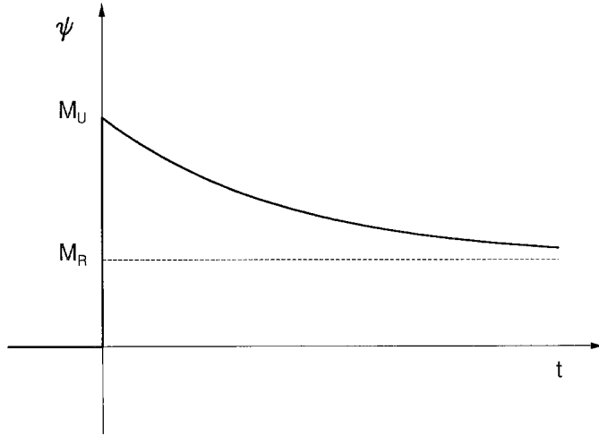
Fig. 17 The relaxation function of the standard linear solid presents an instantaneous unrelaxed state, and at the end of the process the system has relaxed completely to the relaxed modulus M_R .
