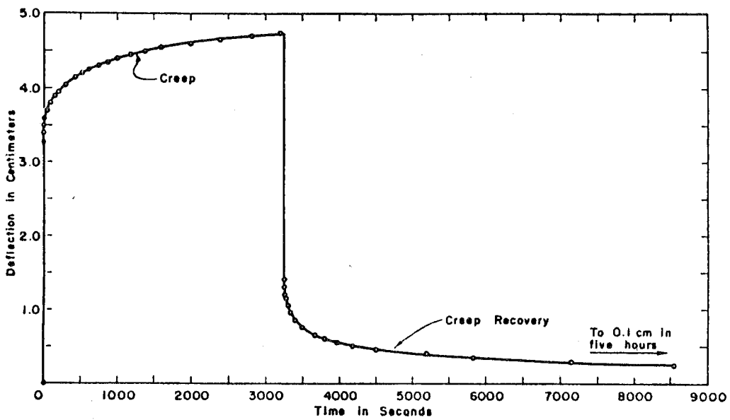
Fig. 2 — Creep function under constant stress and creep recovery in polycrystalline aluminium (Zener, 1948).
