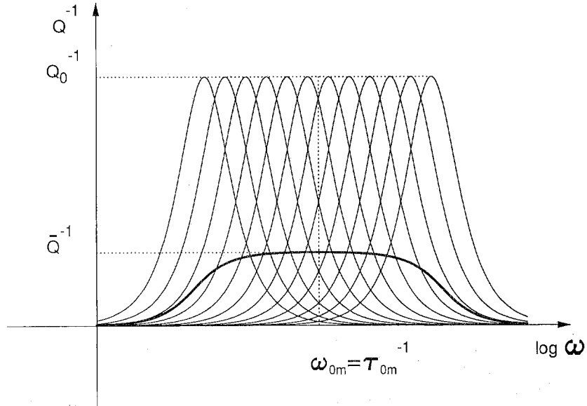
Fig. 21 — A constant- Q model can be constructed with a parallel connection of standard linear solid elements. In this case Q \gg 1 , the system is composed of L relaxation peaks of maximum value Q_0^{-1} each, and equally distributed in the \log(\omega) scale. The algorithm is outlined in Appendix B.
